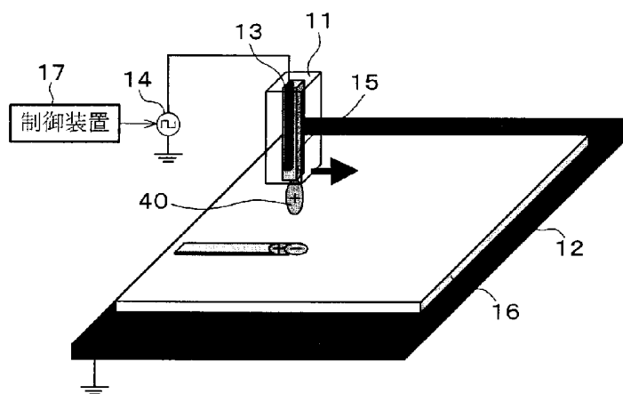
17 CONTROL UNIT
