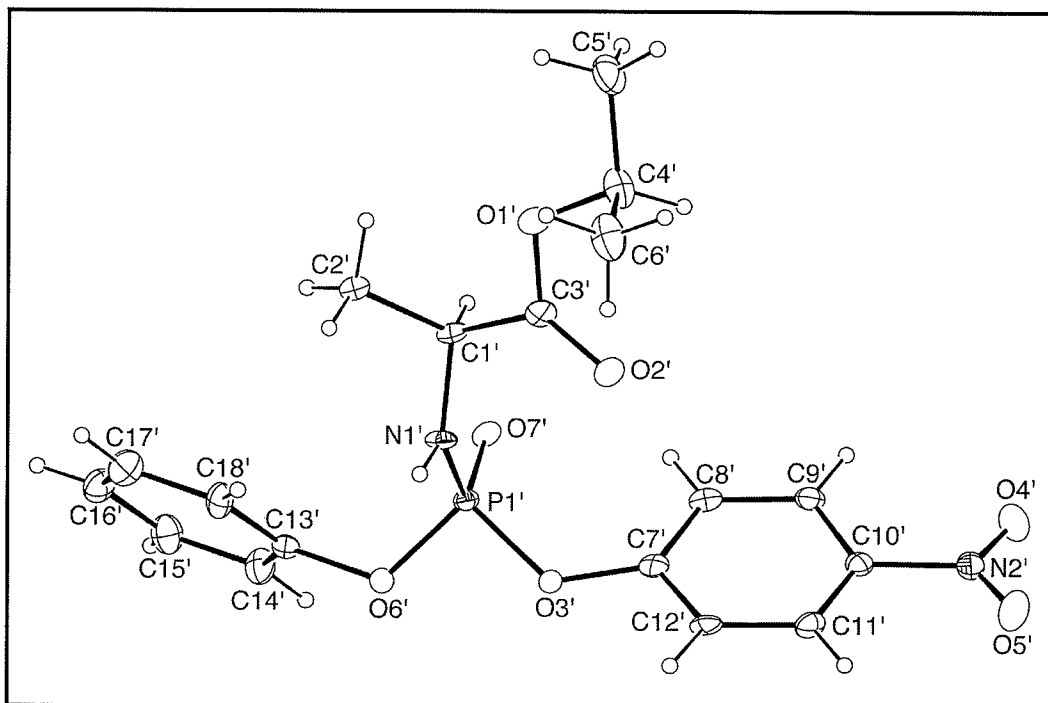
Figure 1B. ORTEP drawing of molecule no. 2 109 of the asymmetric unit with 30% probability thermal ellipsoids.
