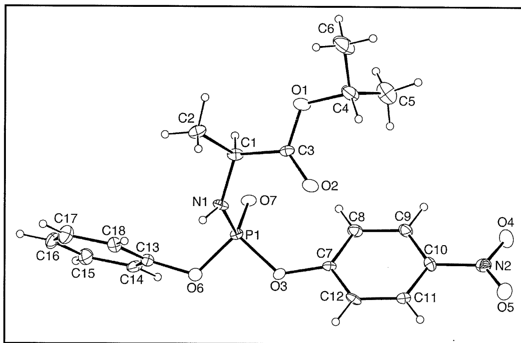
Figure 1A. ORTEP drawing of molecule no. 1 109 of the asymmetric unit with 30% probability thermal ellipsoids.
