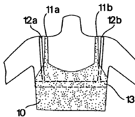
Fig. 1C PRIOR ART
