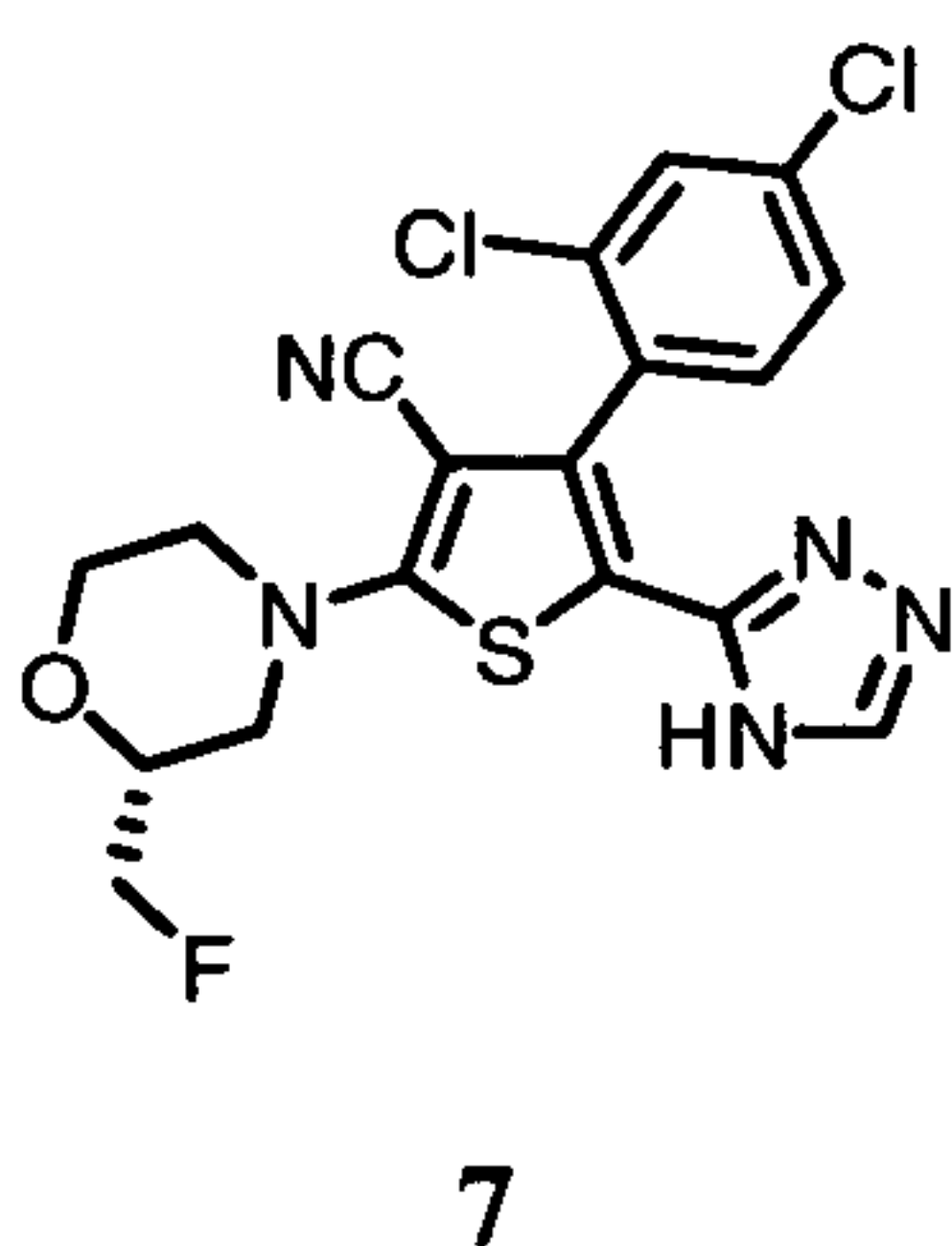
4-(2,4-dichlorophenyl)-2-[(2R)-2-(fluoromethyl)morpholin-4-yl]-5-(4H-1,2,4-triazol-3-yl)thiophene-3-carbonitrile
