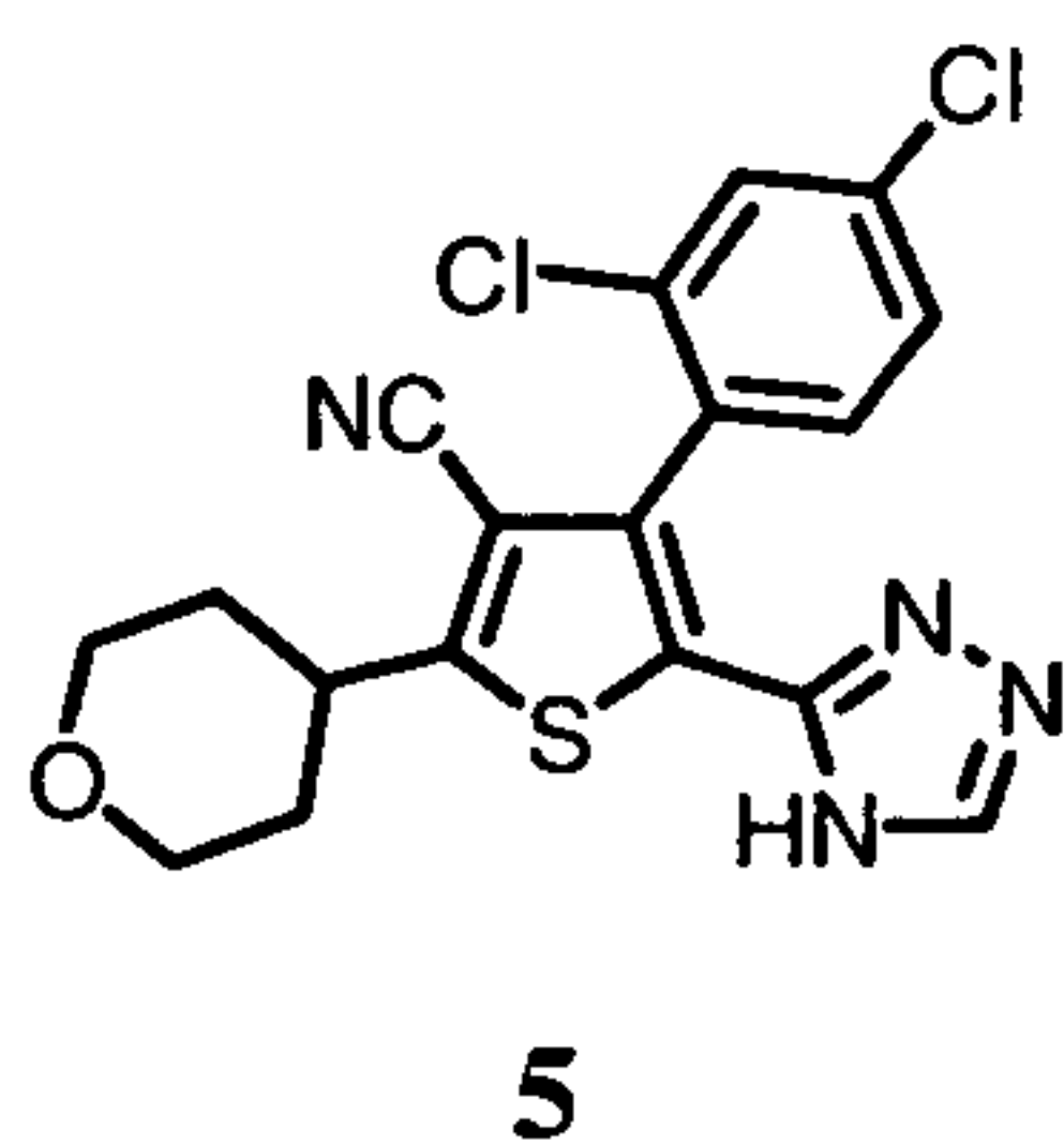
4-(2,4-dichlorophenyl)-2-(tetrahydro-2H-pyran-4-yl)-5-(4H-1,2,4-triazol-3-yl)thiophene-3-carbonitrile
