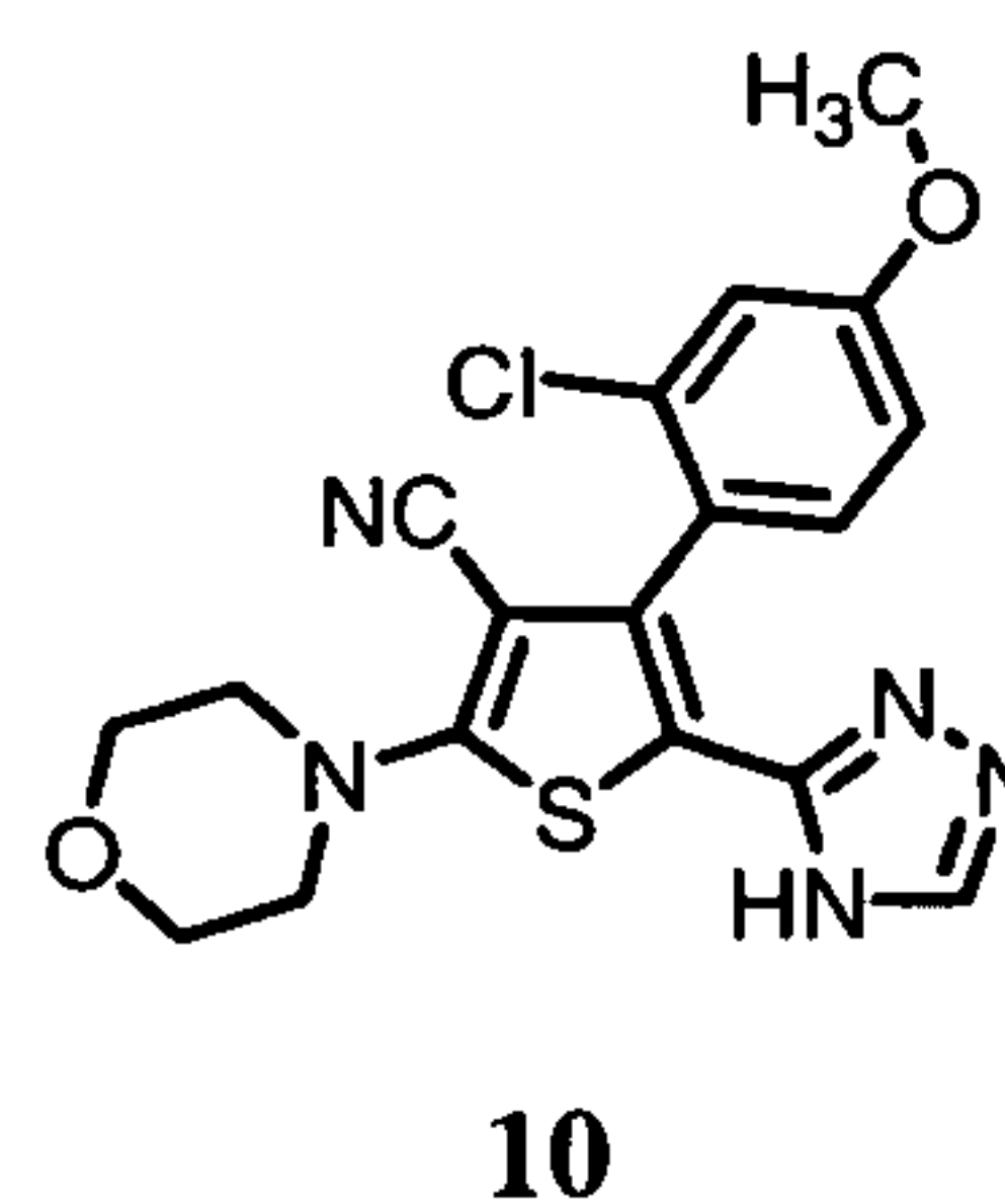
4-(2-chloro-4-methoxyphenyl)-2-morpholin-4-yl-5-(4H-1,2,4-triazol-3-yl)thiophene-3-carbonitrile
