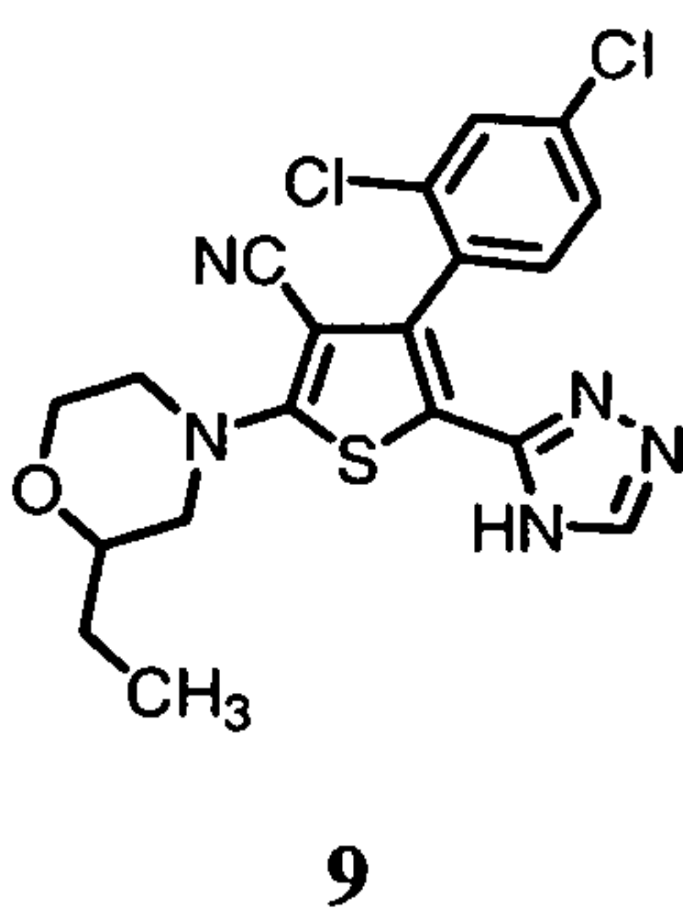
4-(2,4-dichlorophenyl)-2-(2-ethylmorpholin-4-yl)-5-(4H-1,2,4-triazol-3-yl)thiophene-3-carbonitrile
