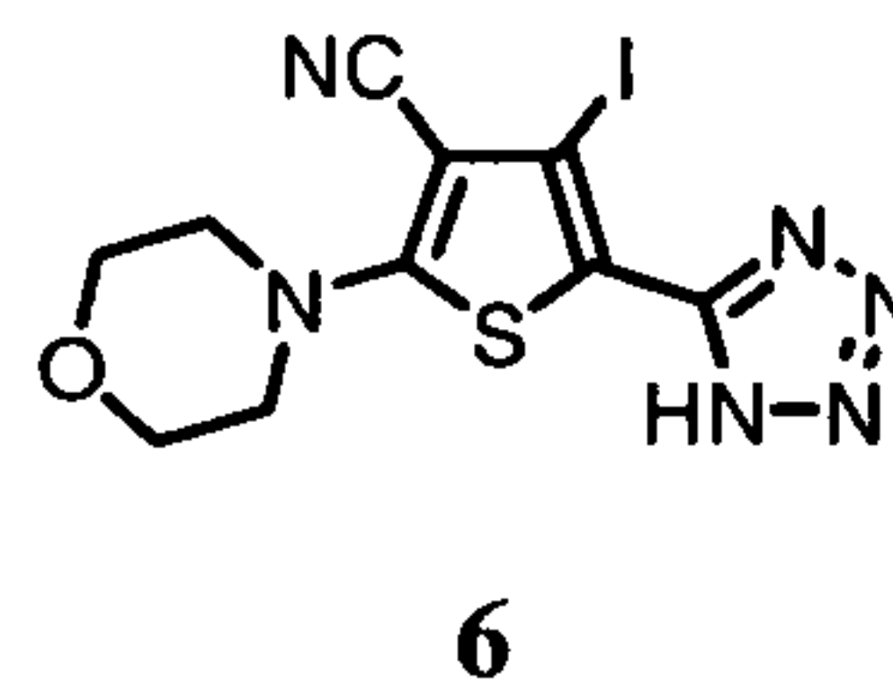
4-iodo-2-morpholin-4-yl-5-(1H-tetrazol-5-yl)thiophene-3-carbonitrile
