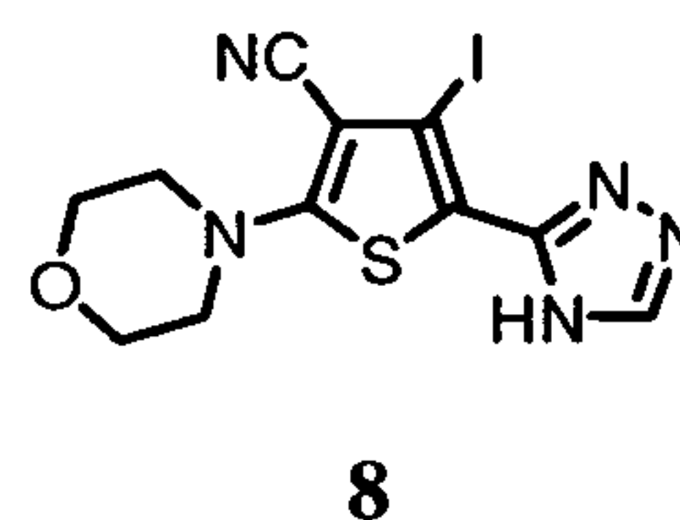
4-iodo-2-morpholin-4-yl-5-(4H-1,2,4-triazol-3-yl)thiophene-3-carbonitrile
