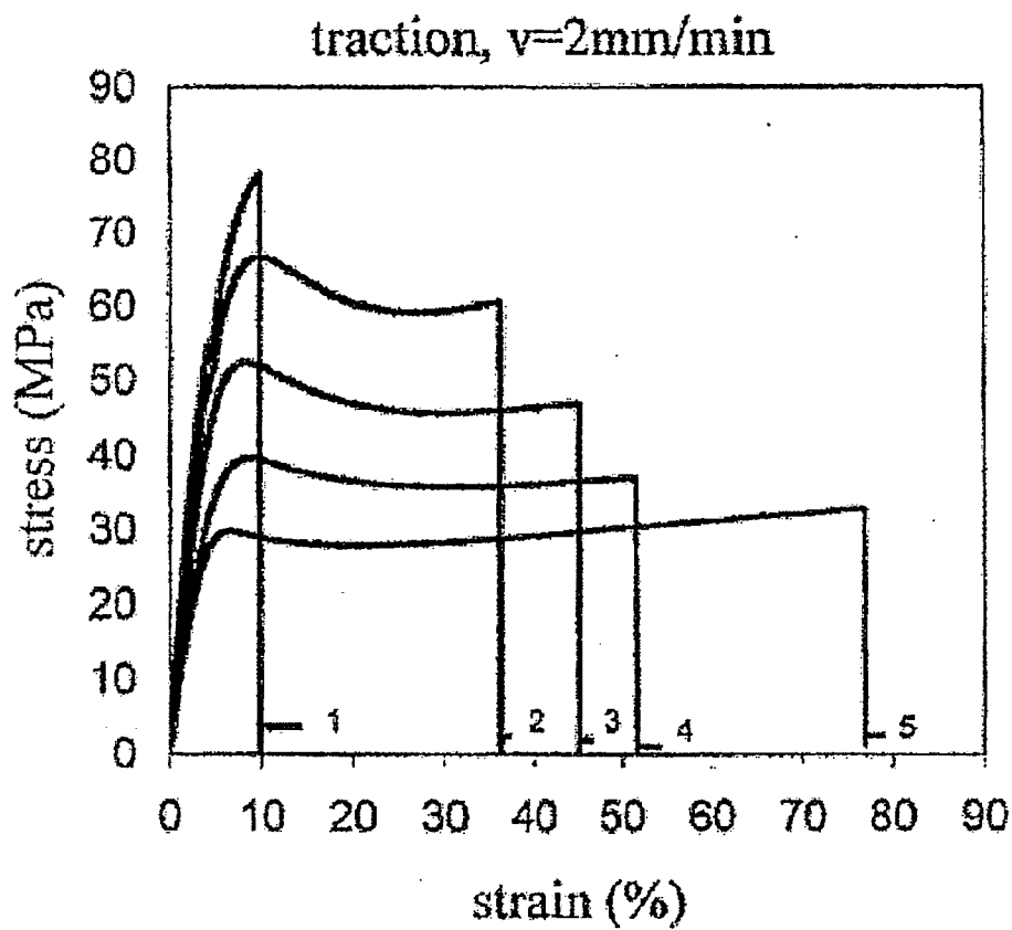
Figure 1 : Traction-elongation test
