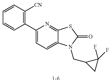
2-(1-{[2,2-difluorocyclopropyl]methyl}-2-oxo-1,2-dihydro[1,3]thiazolo[5,4-b]pyridin-5-yl)benzonitrile (1-6)
