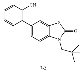
2-[3-(2,2-dimethylpropyl)-2-oxo-2,3-dihydro-1,3-benzothiazol-6-yl]benzonitrile (7-2)
