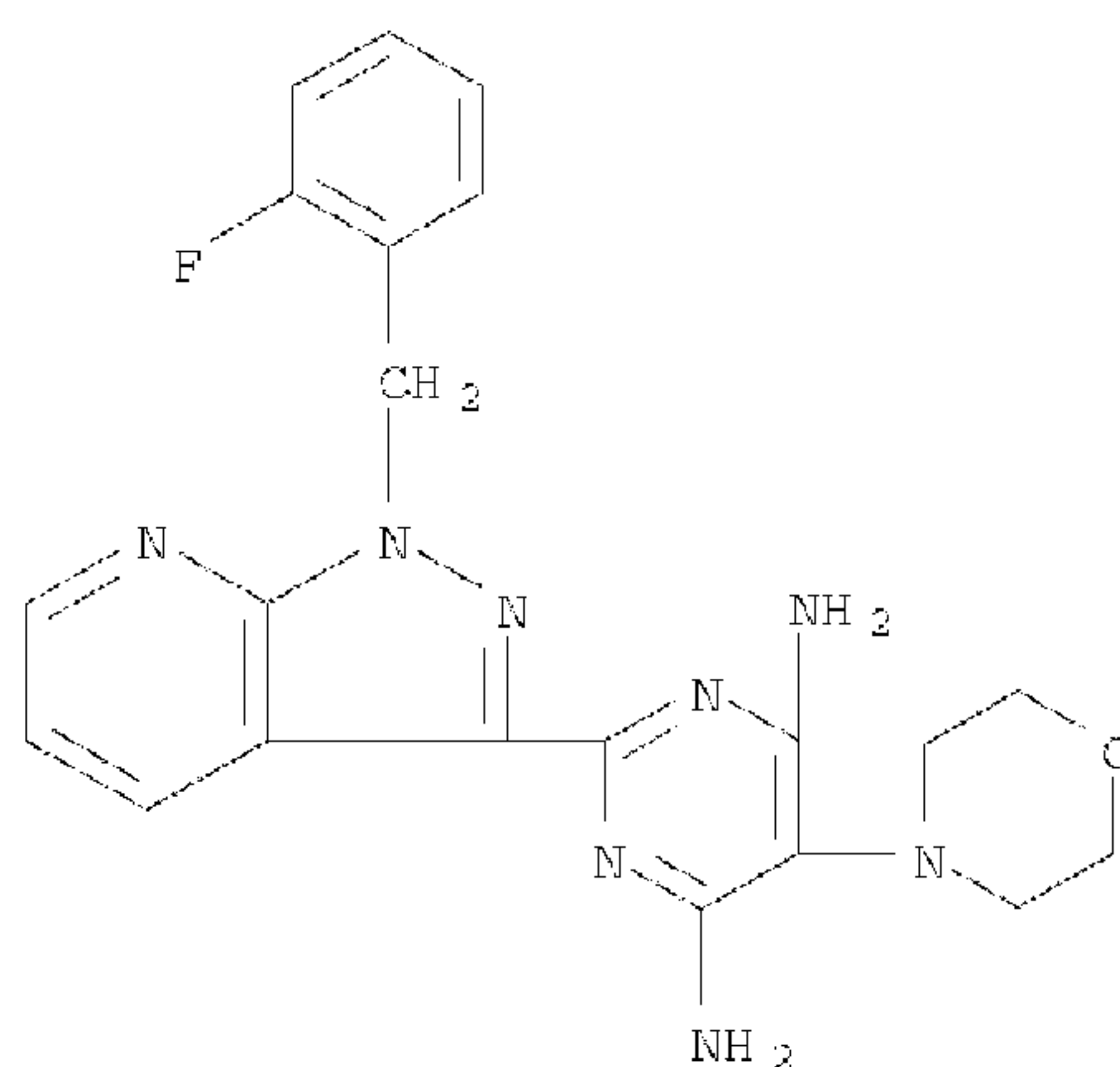
BAY 41-8543 (described in DE19834044)
