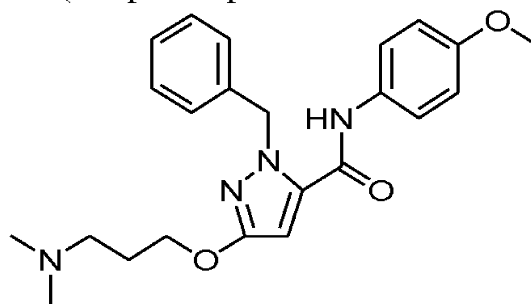
CFM-1571 (see patent publication WO2000027394)
