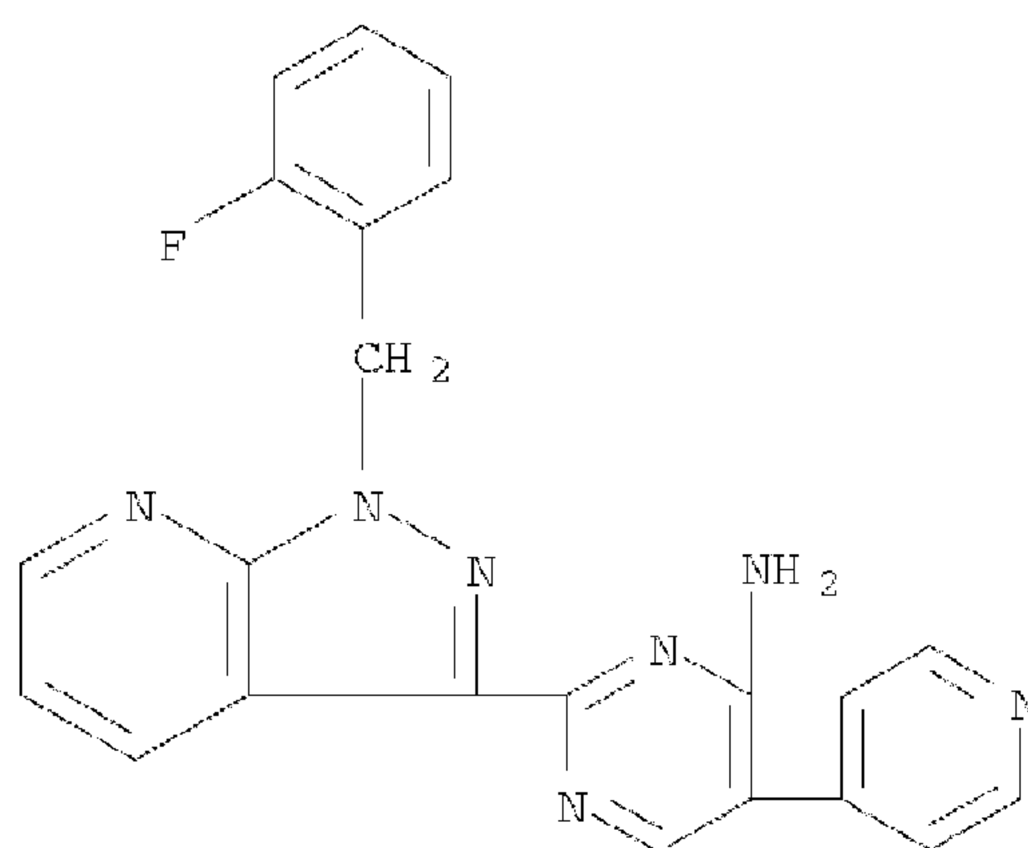
Etricitrat (described in WO 2003086407)
