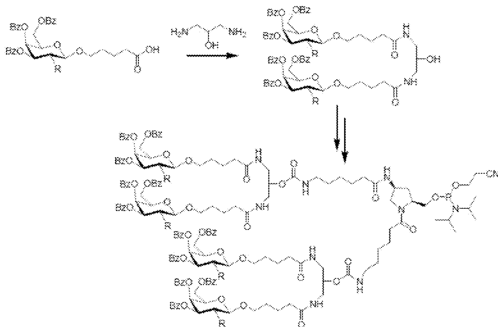
Figure 26. Carbohydrate (GalNAC) clusters for conjugation to siRNA
