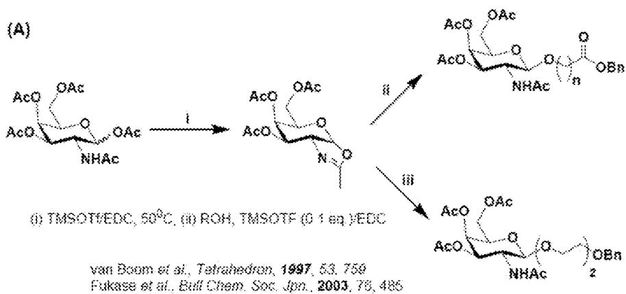
Figure 23. Synthesis of GalNAc building blocks
