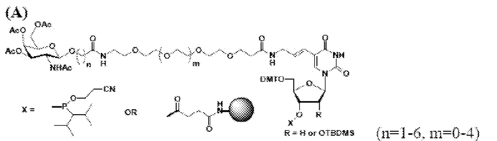
Figure 22. Monomers for carbohydrate conjugation to siRNA
