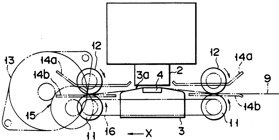
FIG. 1 (PRIOR ART)
