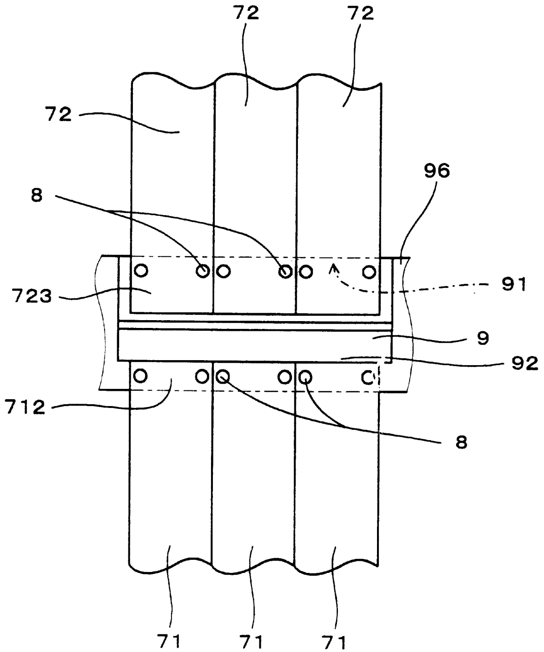
FIG. 9 PRIOR ART
