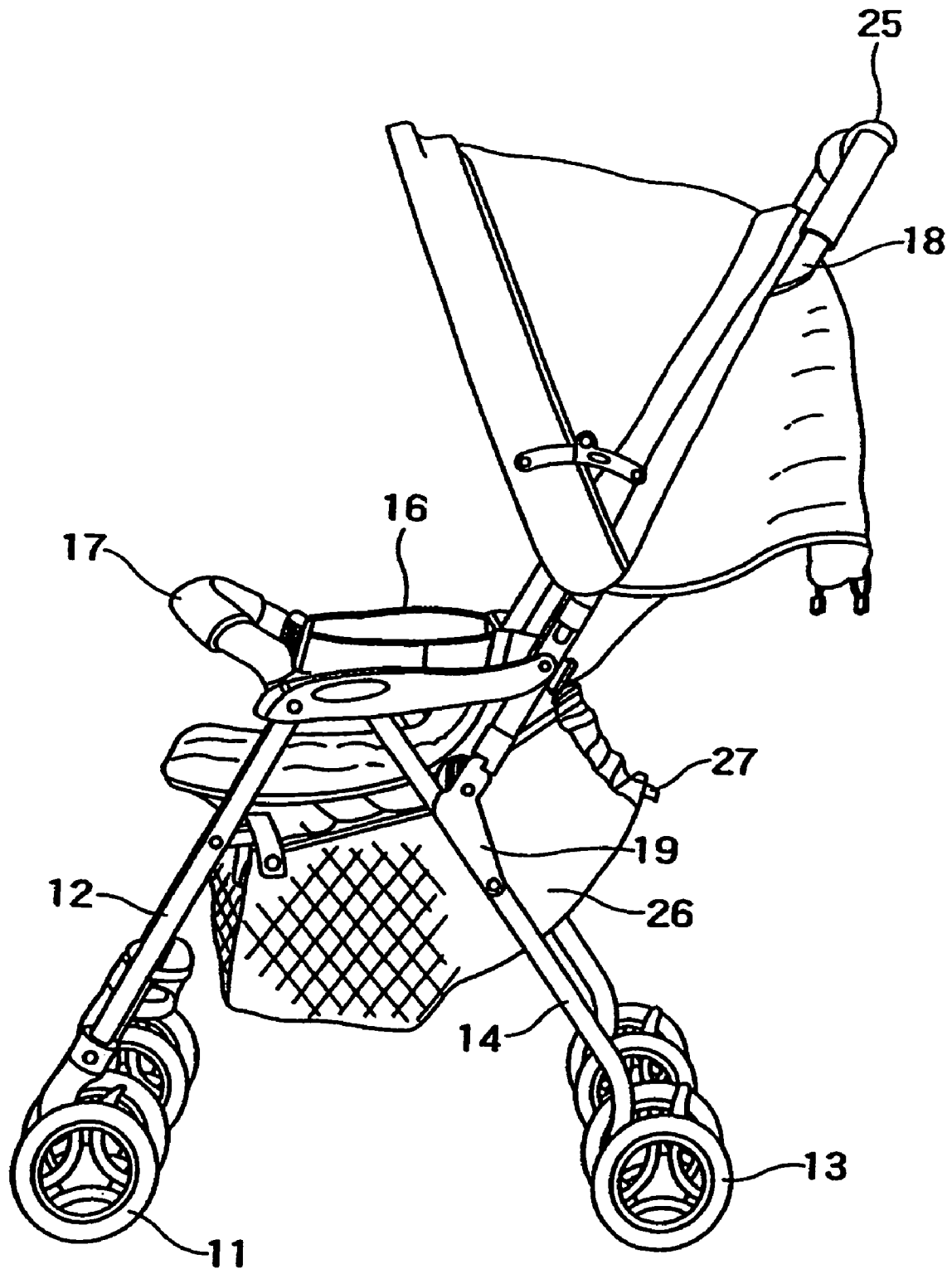
FIG. 16 (PRIOR ART)
