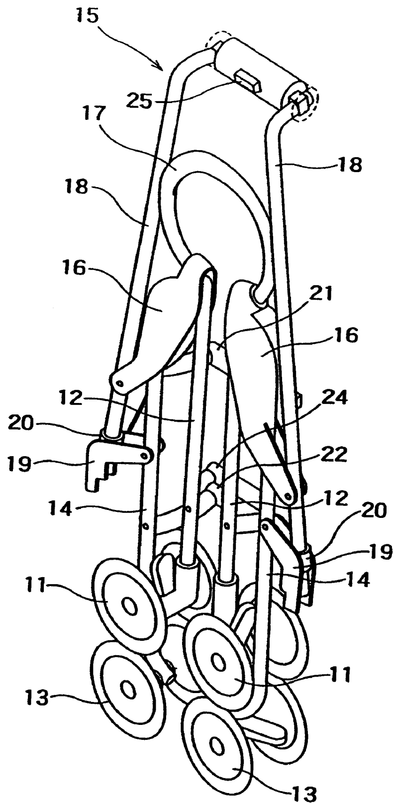
FIG. 15 (PRIOR ART)
