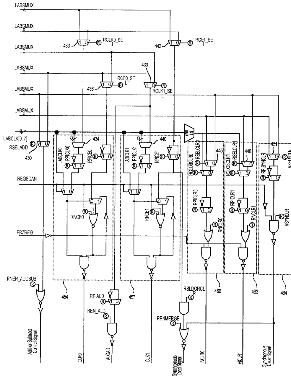
Secondary Signal Generation Unit
