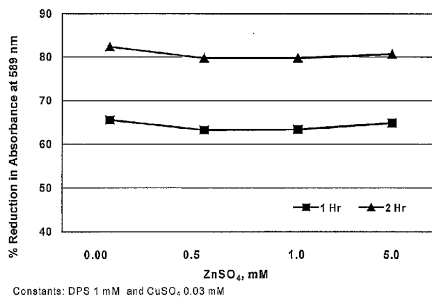
Figure 2: Effect of Zinc Sulfate On Oxidation Performance Of DPS
