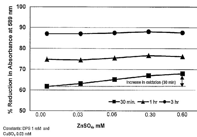
Figure 3: Synergistic Effect of Copper Sulfate and Zinc Sulfate On Oxidation Performance Of DPS
