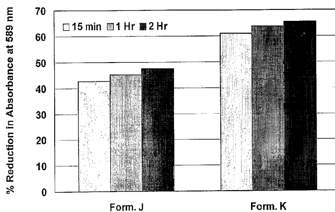
Figure 5: Effect of Copper Sulfate and Copper Sulfate + Zinc Sulfate On Oxidation Performance of Multi-Component Water Treatment Formulations
