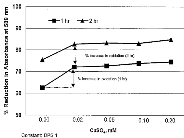
Figure 1: Effect of Copper Sulfate On Oxidation Performance Of DPS
