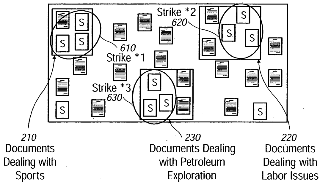
Implicit Location of Derived Word Senses FIG. 9
