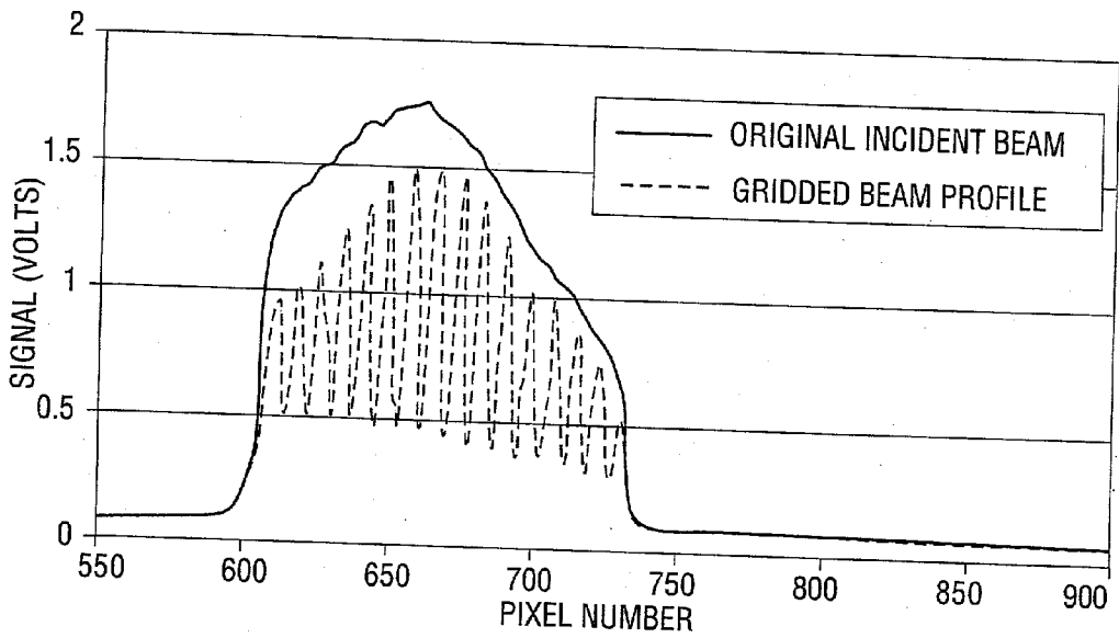
INCIDENT BEAM PROFILE FORMED BY A GRID MASK
