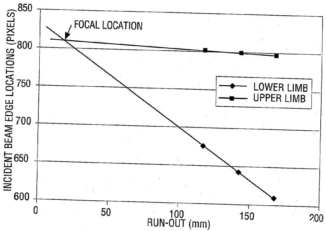
DETERMINING THE FOCAL LOCATION FIG. 7
