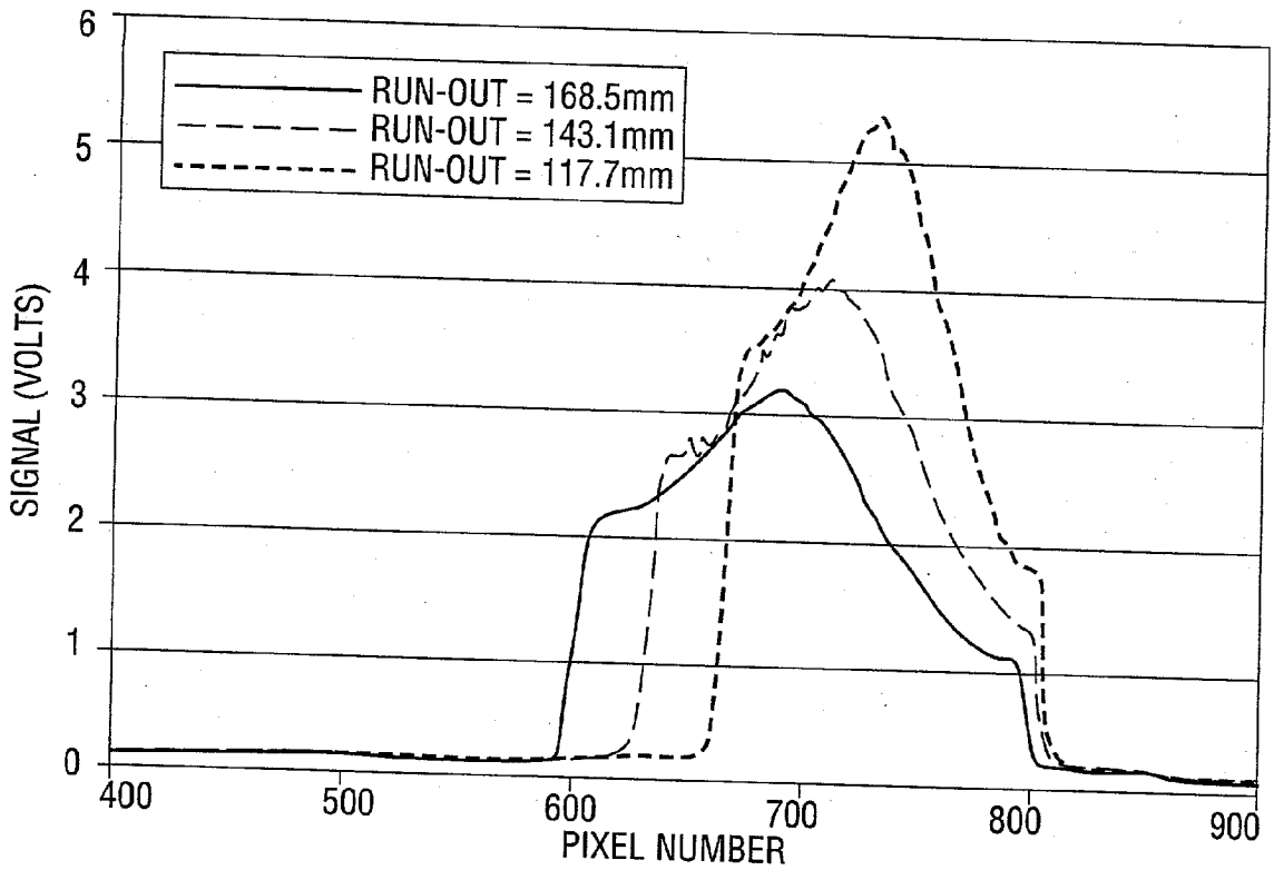
INCIDENT BEAM PROFILES AT DIFFERENT RUN-OUT DISTANCES FIG. 6
