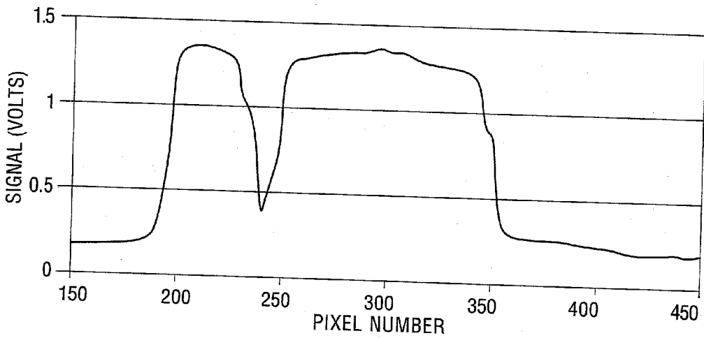
SHADOW OF A FINE WIRE IN AN INCIDENT BEAM PROFILE
