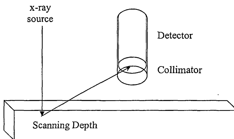
Exemplary Geometrical Focusing Schematic
