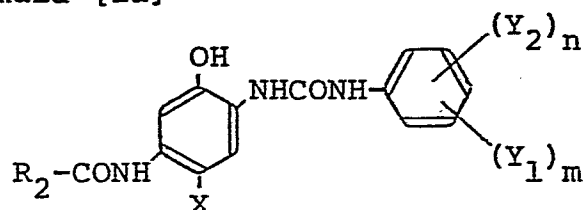
Formula [Ia]
