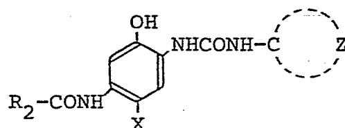
Formula [Ib]
