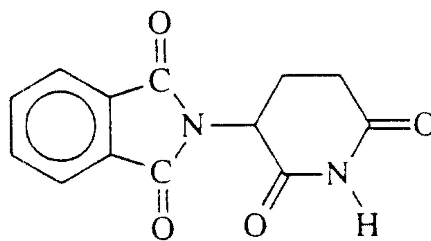
thalidomide
