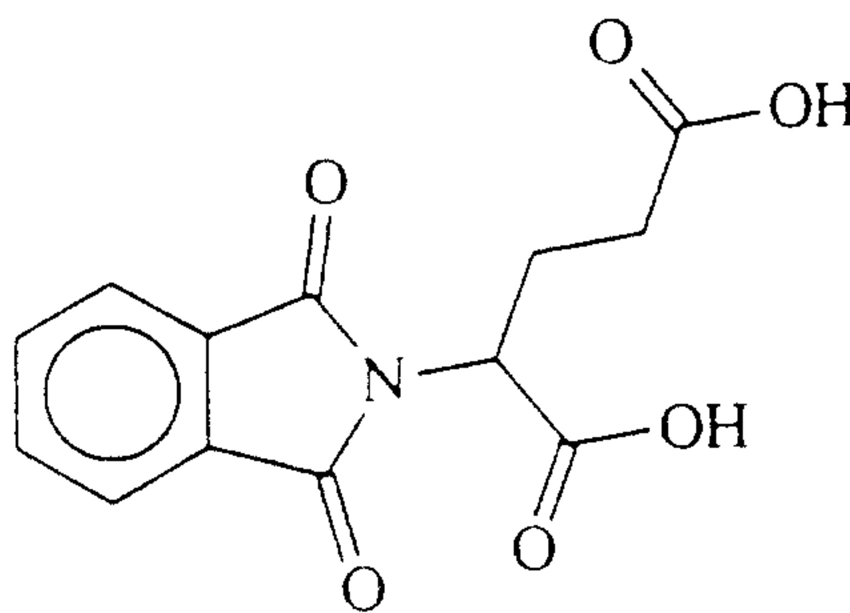
phthaloyl glutamic acid (PG Acid)
