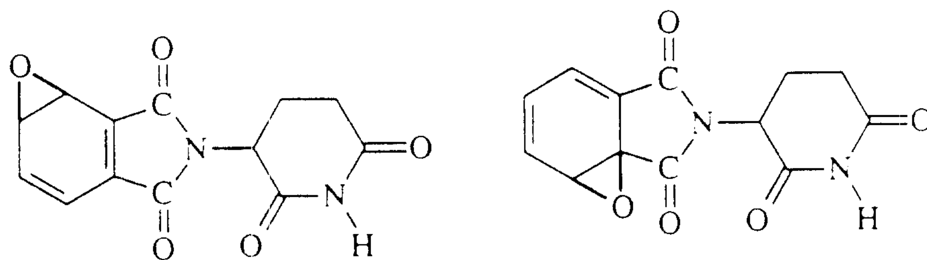
Epoxides of thalidomide
