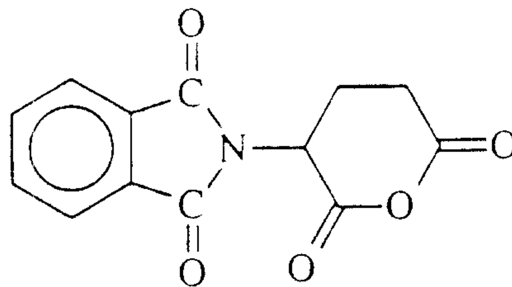
phthaloyl glutamic anhydride (PGA)
