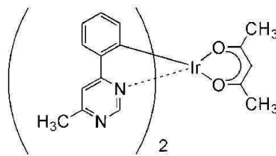
[Ir(mppm) 2 (acac)]
