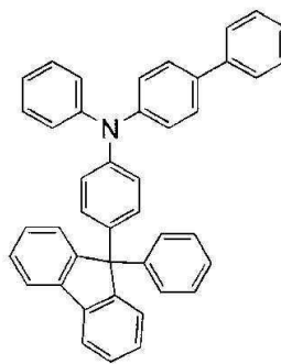
BPAFLP
