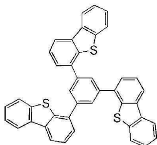
DBT3P-II
