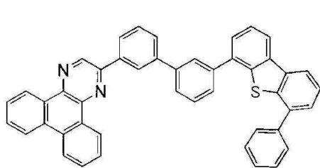
2mDBTBPDBq-IV
