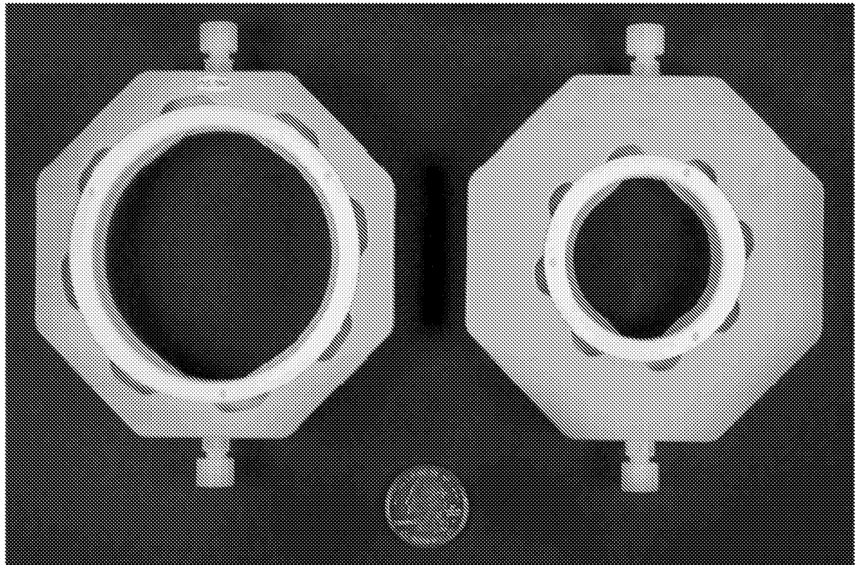
LEFT CELL 63.5 mm Housing Clearance Diameter, 1.6 mm Thick / 76.2 mm Diameter Windows
