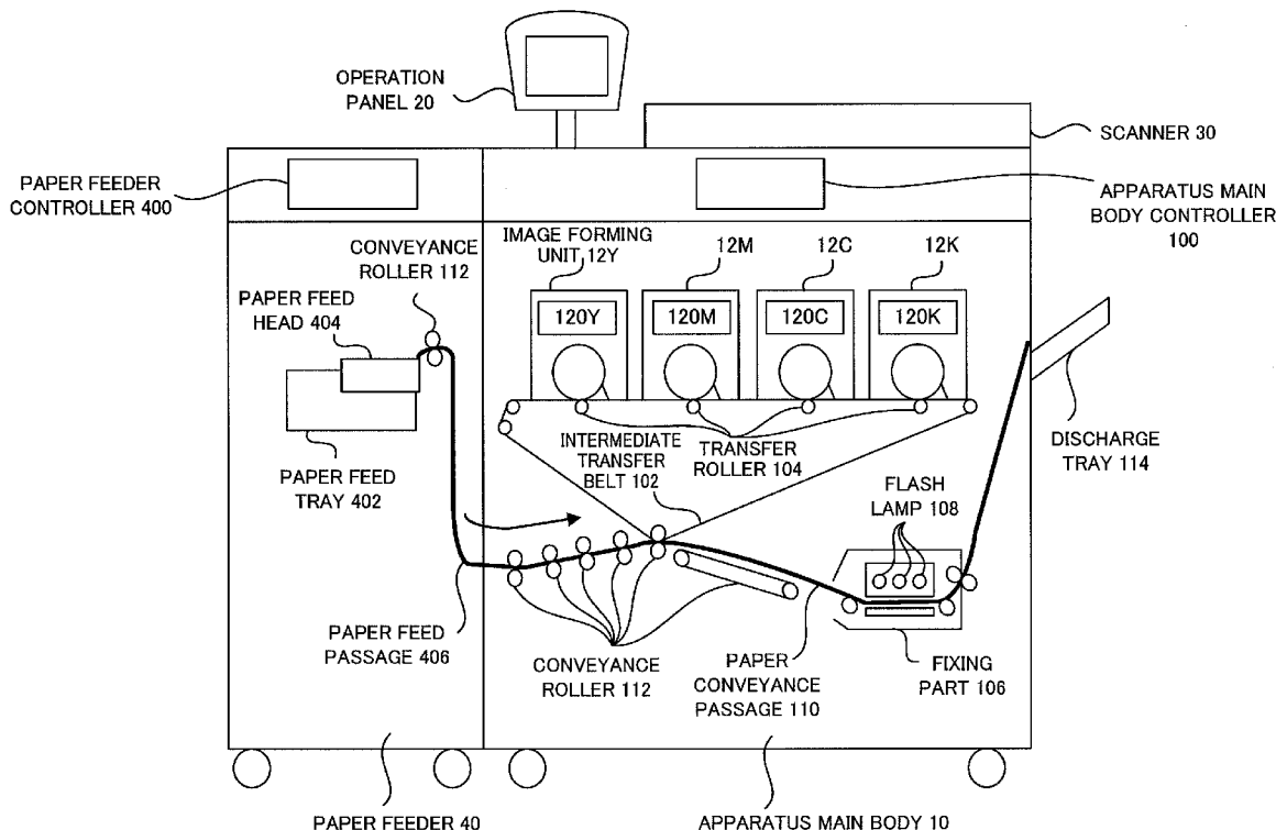
IMAGE FORMING APPARATUS 1
