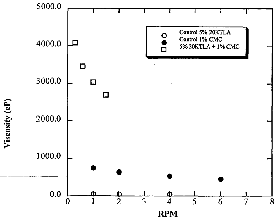
Figure 4 Viscosity of 5% 20KTLA with 1% CMC
