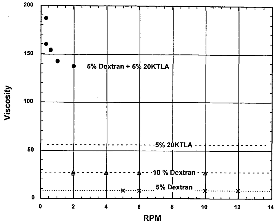
Figure 7. Viscosities of 20KTLA – Dextran Mixtures
