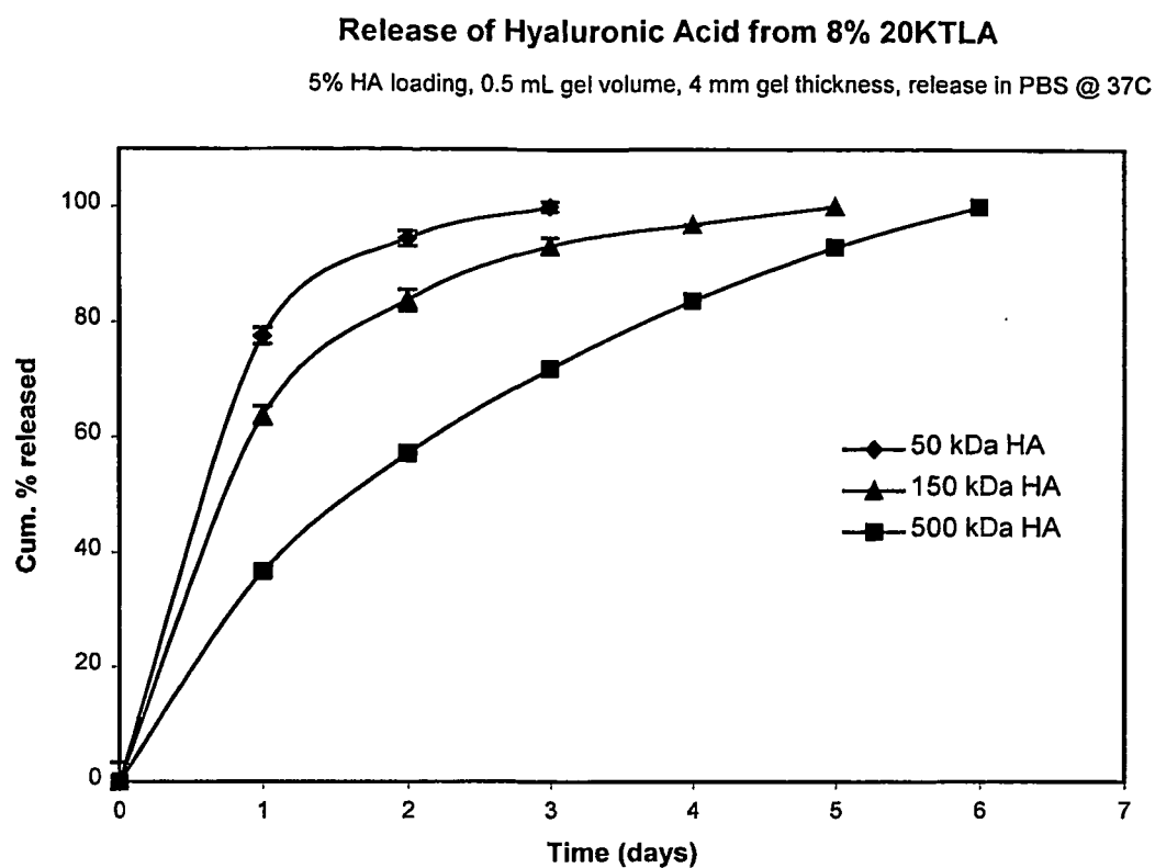
FIGURE 9. HA Release from 8% 20KTLA
