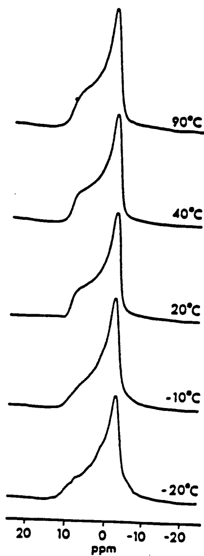
FIG. 1 ^{31}\text{P} -NMR SPECTRA OF LOPE AT pH 7
