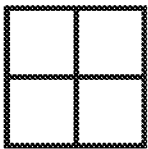
Max Pool
