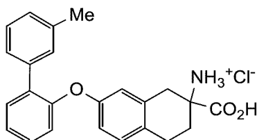
2-carboxy-7-((3'-methyl-[1,1'-biphenyl]-2-yl)oxy)-1,2,3,4-tetrahydronaphthalene-2-aminium chloride
