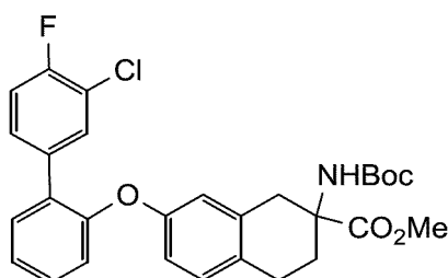
methyl 2-((tert-butoxycarbonyl)amino)-7-((3'-chloro-4'-fluoro-[1,1'-biphenyl]-2-yl)oxy)-1,2,3,4-tetrahydronaphthalene-2-carboxylate
