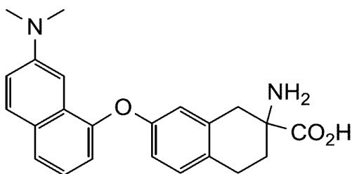
2-amino-7-((7-(dimethylamino)naphthalen-1-yl)oxy)-1,2,3,4-tetrahydronaphthalene-2-carboxylic acid
