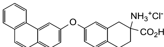
2-carboxy-7-(phenanthren-3-yloxy)-1,2,3,4-tetrahydronaphthalen-2-aminium chloride
