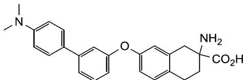
2-amino-7-((4'-(dimethylamino)-[1,1'-biphenyl]-3-yl)oxy)-1,2,3,4-tetrahydronaphthalene-2-carboxylic acid
