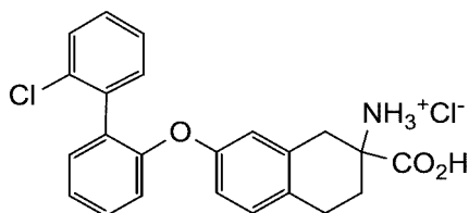
2-carboxy-7-((2'-chloro-[1,1'-biphenyl]-2-yl)oxy)-1,2,3,4-tetrahydronaphthalene-2-aminium chloride
