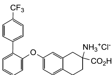
2-carboxy-7-((4'-(trifluoromethyl)-[1,1'-biphenyl]-2-yl)oxy)-1,2,3,4-tetrahydronaphthalen-2-aminium chloride
