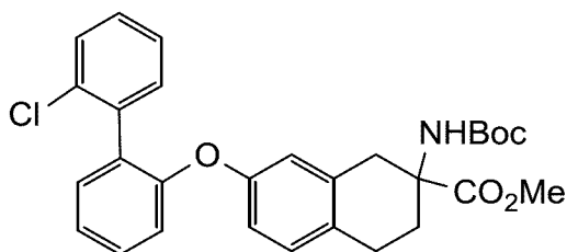
methyl 2-((tert-butoxycarbonyl)amino)-7-((2'-chloro-[1,1'-biphenyl]-2-yl)oxy)-1,2,3,4-tetrahydronaphthalene-2-carboxylate
