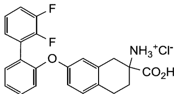
2-carboxy-7-((2',3'-difluoro-[1,1'-biphenyl]-2-yl)oxy)-1,2,3,4-tetrahydronaphthalen-2-aminium chloride
