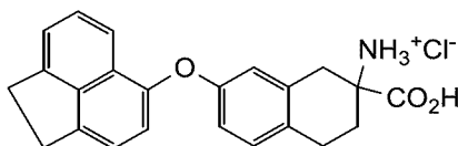
2-carboxy-7-((1,2-dihydroacenaphthylen-5-yl)oxy)-1,2,3,4-tetrahydronaphthalen-2-aminium chloride
