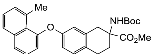
methyl 2-((tert-butoxycarbonyl)amino)-7-((8-methylnaphthalen-1-yl)oxy)-1,2,3,4-tetrahydronaphthalene-2-carboxylate
