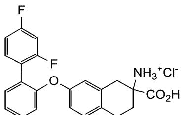
2-carboxy-7-((2',4'-difluoro-[1,1'-biphenyl]-2-yl)oxy)-1,2,3,4-tetrahydronaphthalen-2-aminium chloride
