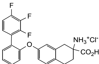
2-carboxy-7-((2',3',4'-trifluoro-[1,1'-biphenyl]-2-yl)oxy)-1,2,3,4-tetrahydronaphthalen-2-aminium chloride
