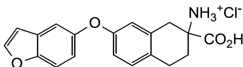
7-(benzofuran-5-yloxy)-2-carboxy-1,2,3,4-tetrahydronaphthalen-2-aminium chloride
