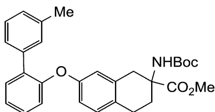
methyl 2-((tert-butoxycarbonyl)amino)-7-((3'-methyl-[1,1'-biphenyl]-2-yl)oxy)-1,2,3,4-tetrahydronaphthalene-2-carboxylate
