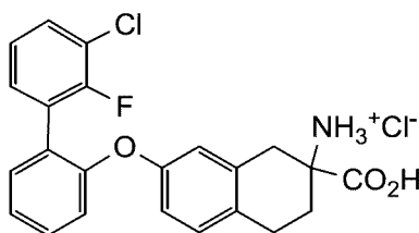
2-carboxy-7-((3'-chloro-2'-fluoro-[1,1'-biphenyl]-2-yl)oxy)-1,2,3,4-tetrahydronaphthalen-2-aminium chloride
