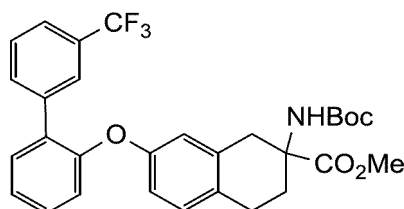
methyl 2-((tert-butoxycarbonyl)amino)-7-((3'-(trifluoromethyl)-[1,1'-biphenyl]-2-yl)oxy)-1,2,3,4-tetrahydronaphthalene-2-carboxylate
