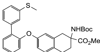
methyl 2-((tert-butoxycarbonyl)amino)-7-((3'-(methylthio)-[1,1'-biphenyl]-2-yl)oxy)-1,2,3,4-tetrahydronaphthalene-2-carboxylate
