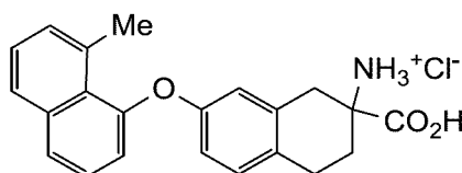
2-carboxy-7-((8-methylnaphthalen-1-yl)oxy)-1,2,3,4-tetrahydronaphthalen-2-aminium chloride
