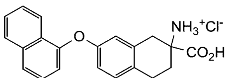
2-carboxy-7-(naphthalen-1-yloxy)-1,2,3,4-tetrahydronaphthalen-2-aminium chloride
