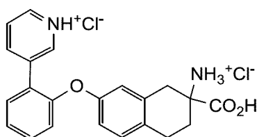
3-(2-((7-ammonio-7-carboxy-5,6,7,8-tetrahydronaphthalen-2-yl)oxy)phenyl)pyridin-1-ium chloride
