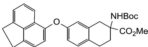
methyl 2-((tert-butoxycarbonyl)amino)-7-((1,2-dihydroacenaphthylen-5-yl)oxy)-1,2,3,4-tetrahydronaphthalene-2-carboxylate
