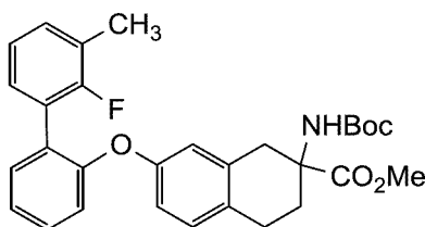
methyl 2-((tert-butoxycarbonyl)amino)-7-((2'-fluoro-3'-methyl-[1,1'-biphenyl]-2-yl)oxy)-1,2,3,4-tetrahydronaphthalene-2-carboxylate
