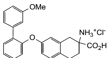
2-carboxy-7-((3'-methoxy-[1,1'-biphenyl]-2-yl)oxy)-1,2,3,4-tetrahydronaphthalene-2-aminium chloride
