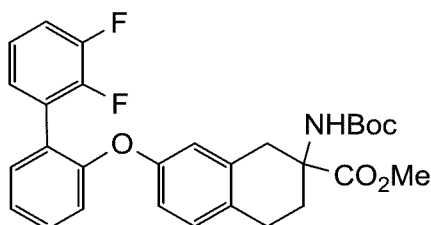
methyl 2-((tert-butoxycarbonyl)amino)-7-((2',3'-difluoro-[1,1'-biphenyl]-2-yl)oxy)-1,2,3,4-tetrahydronaphthalene-2-carboxylate
