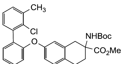
methyl 2-((tert-butoxycarbonyl)amino)-7-((2'-chloro-3'-methyl-[1,1'-biphenyl]-2-yl)oxy)-1,2,3,4-tetrahydronaphthalene-2-carboxylate
