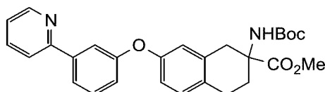
methyl 2-((tert-butoxycarbonyl)amino)-7-(3-(pyridin-2-yl)phenoxy)-1,2,3,4-tetrahydronaphthalene-2-carboxylate
