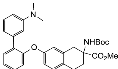
methyl 2-((tert-butoxycarbonyl)amino)-7-((3'-(dimethylamino)-[1,1'-biphenyl]-2-yl)oxy)-1,2,3,4-tetrahydronaphthalene-2-carboxylate
