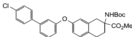
methyl 2-((tert-butoxycarbonyl)amino)-7-((4'-chloro-[1,1'-biphenyl]-3-yl)oxy)-1,2,3,4-tetrahydronaphthalene-2-carboxylate
