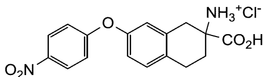
2-carboxy-7-(4-nitrophenoxy)-1,2,3,4-tetrahydronaphthalen-2-aminium chloride
