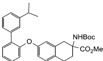
methyl 2-((tert-butoxycarbonyl)amino)-7-((3'-isopropyl-[1,1'-biphenyl]-2-yl)oxy)-1,2,3,4-tetrahydronaphthalene-2-carboxylate
