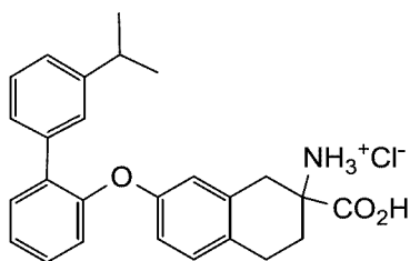
2-carboxy-7-((3'-isopropyl-[1,1'-biphenyl]-2-yl)oxy)-1,2,3,4-tetrahydronaphthalen-2-aminium chloride
