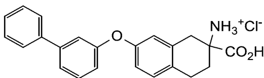
7-([1,1'-biphenyl]-3-yloxy)-2-carboxy-1,2,3,4-tetrahydronaphthalen-2-aminium chloride
