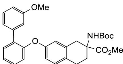
methyl 2-((tert-butoxycarbonyl)amino)-7-((3'-methoxy-[1,1'-biphenyl]-2-yl)oxy)-1,2,3,4-tetrahydronaphthalene-2-carboxylate
