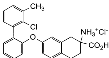
2-carboxy-7-((2'-chloro-3'-methyl-[1,1'-biphenyl]-2-yl)oxy)-1,2,3,4-tetrahydronaphthalen-2-aminium chloride
