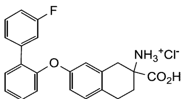
2-carboxy-7-((3'-fluoro-[1,1'-biphenyl]-2-yl)oxy)-1,2,3,4-tetrahydronaphthalen-2-aminium chloride
