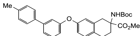
methyl 2-((tert-butoxycarbonyl)amino)-7-((4'-methyl-[1,1'-biphenyl]-3-yl)oxy)-1,2,3,4-tetrahydronaphthalene-2-carboxylate
