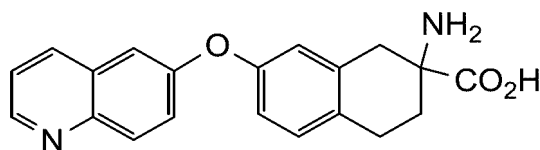
2-amino-7-(quinolin-6-yloxy)-1,2,3,4-tetrahydronaphthalene-2-carboxylic acid
