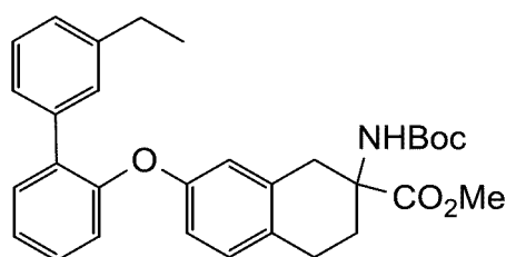
methyl 2-((tert-butoxycarbonyl)amino)-7-((3'-ethyl-[1,1'-biphenyl]-2-yl)oxy)-1,2,3,4-tetrahydronaphthalene-2-carboxylate
