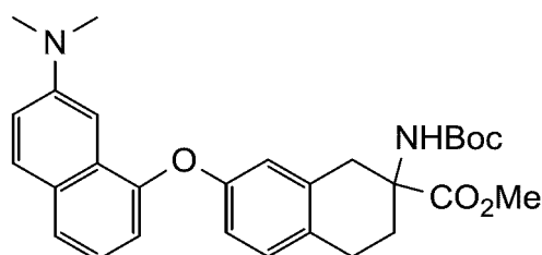
methyl 2-((tert-butoxycarbonyl)amino)-7-((7-(dimethylamino)naphthalen-1-yl)oxy)-1,2,3,4-tetrahydronaphthalene-2-carboxylate
