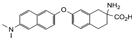
2-amino-7-((6-(dimethylamino)naphthalen-2-yl)oxy)-1,2,3,4-tetrahydronaphthalene-2-carboxylic acid
