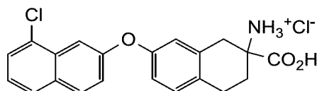
2-carboxy-7-((8-chloronaphthalen-2-yl)oxy)-1,2,3,4-tetrahydronaphthalen-2-aminium chloride
