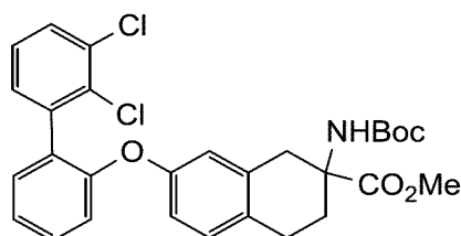
methyl 2-((tert-butoxycarbonyl)amino)-7-((2',3'-dichloro-[1,1'-biphenyl]-2-yl)oxy)-1,2,3,4-tetrahydronaphthalene-2-carboxylate
