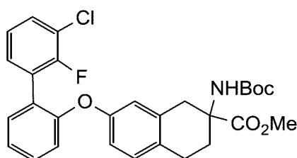
methyl 2-((tert-butoxycarbonyl)amino)-7-((3'-chloro-2'-fluoro-[1,1'-biphenyl]-2-yl)oxy)-1,2,3,4-tetrahydronaphthalene-2-carboxylate
