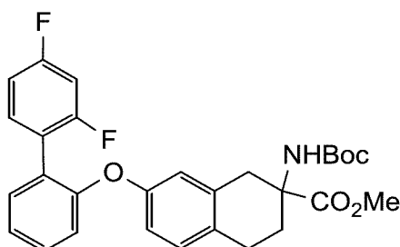
methyl 2-((tert-butoxycarbonyl)amino)-7-((2',4'-difluoro-[1,1'-biphenyl]-2-yl)oxy)-1,2,3,4-tetrahydronaphthalene-2-carboxylate
