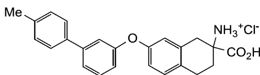
2-carboxy-7-((4'-methyl-[1,1'-biphenyl]-3-yl)oxy)-1,2,3,4-tetrahydronaphthalen-2-aminium chloride
