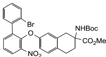
methyl 7-((2'-bromo-3-nitro-[1,1'-biphenyl]-2-yl)oxy)-2-((tert-butoxycarbonyl)amino)-1,2,3,4-tetrahydronaphthalene-2-carboxylate
