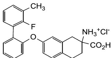
2-carboxy-7-((2'-fluoro-3'-methyl-[1,1'-biphenyl]-2-yl)oxy)-1,2,3,4-tetrahydronaphthalen-2-aminium chloride
