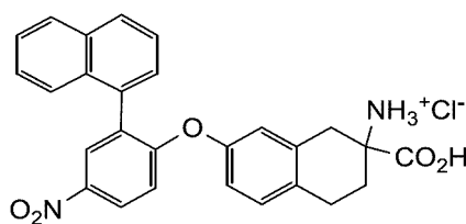
2-carboxy-7-(2-(naphthalen-1-yl)-4-nitrophenoxy)-1,2,3,4-tetrahydronaphthalen-2-aminium chloride
