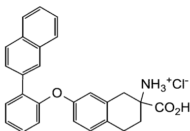
2-carboxy-7-(2-(naphthalen-2-yl)phenoxy)-1,2,3,4-tetrahydronaphthalen-2-aminium chloride
