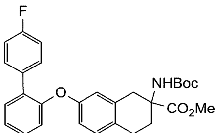
methyl 2-((tert-butoxycarbonyl)amino)-7-((4'-fluoro-[1,1'-biphenyl]-2-yl)oxy)-1,2,3,4-tetrahydronaphthalene-2-carboxylate
