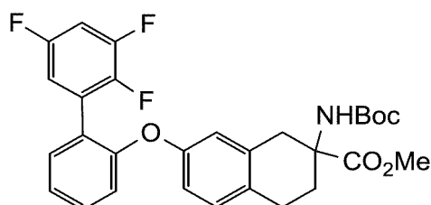
methyl 2-((tert-butoxycarbonyl)amino)-7-((2',3',5'-trifluoro-[1,1'-biphenyl]-2-yl)oxy)-1,2,3,4-tetrahydronaphthalene-2-carboxylate
