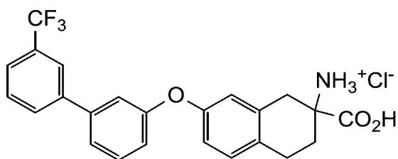
2-carboxy-7-((3'-(trifluoromethyl)-[1,1'-biphenyl]-3-yl)oxy)-1,2,3,4-tetrahydronaphthalen-2-aminium chloride
