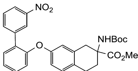
methyl 2-((tert-butoxycarbonyl)amino)-7-((3'-nitro-[1,1'-biphenyl]-2-yl)oxy)-1,2,3,4-tetrahydronaphthalene-2-carboxylate
