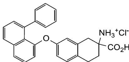
2-carboxy-7-((8-phenylnaphthalen-1-yl)oxy)-1,2,3,4-tetrahydronaphthalen-2-aminium chloride
