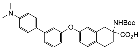
2-((tert-butoxycarbonyl)amino)-7-((4'-(dimethylamino)-[1,1'-biphenyl]-3-yl)oxy)-1,2,3,4-tetrahydronaphthalene-2-carboxylic acid
