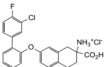
2-carboxy-7-((3'-chloro-4'-fluoro-[1,1'-biphenyl]-2-yl)oxy)-1,2,3,4-tetrahydronaphthalen-2-aminium chloride
