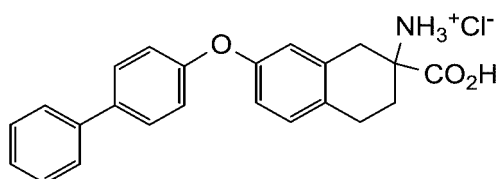
7-([1,1'-biphenyl]-4-yloxy)-2-carboxy-1,2,3,4-tetrahydronaphthalen-2-aminium chloride
