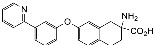
2-amino-7-(3-(pyridin-2-yl)phenoxy)-1,2,3,4-tetrahydronaphthalene-2-carboxylic acid
