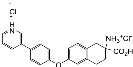
3-(4-((6-ammonio-6-carboxy-5,6,7,8-tetrahydronaphthalen-2-yl)oxy)phenyl)pyridine-1-ium chloride
