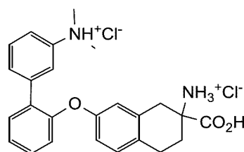
2-carboxy-7-((3'-(dimethylammonio)-[1,1'-biphenyl]-2-yl)oxy)-1,2,3,4-tetrahydronaphthalene-2-ammonium chloride
