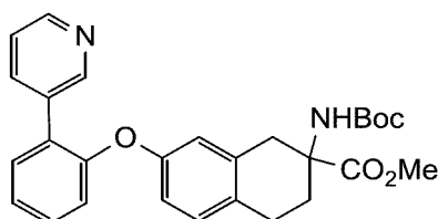
methyl 2-((tert-butoxycarbonyl)amino)-7-(2-(pyridin-3-yl)phenoxy)-1,2,3,4-tetrahydronaphthalene-2-carboxylate
