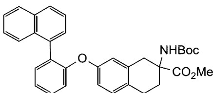
methyl 2-((tert-butoxycarbonyl)amino)-7-(2-(naphthalen-1-yl)phenoxy)-1,2,3,4-tetrahydronaphthalene-2-carboxylate
