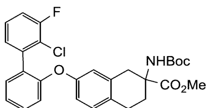
methyl 2-((tert-butoxycarbonyl)amino)-7-((2'-chloro-3'-fluoro-[1,1'-biphenyl]-2-yl)oxy)-1,2,3,4-tetrahydronaphthalene-2-carboxylate
