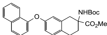
methyl 2-((tert-butoxycarbonyl)amino)-7-(naphthalen-1-yloxy)-1,2,3,4-tetrahydronaphthalene-2-carboxylate
