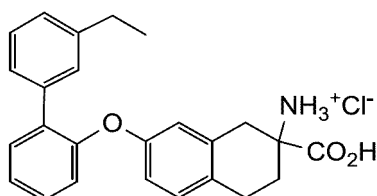
2-carboxy-7-((3'-ethyl-[1,1'-biphenyl]-2-yl)oxy)-1,2,3,4-tetrahydronaphthalene-2-aminium chloride
