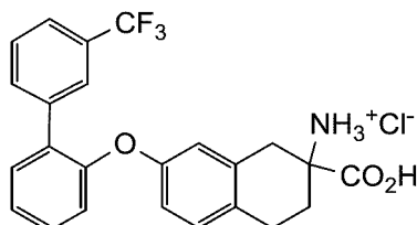
2-carboxy-7-((3'-(trifluoromethyl)-[1,1'-biphenyl]-2-yl)oxy)-1,2,3,4-tetrahydronaphthalen-2-aminium chloride
