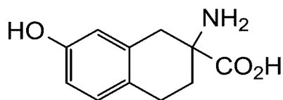
2-amino-7-hydroxy-1,2,3,4-tetrahydronaphthalene-2-carboxylic acid
