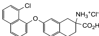
2-carboxy-7-((8-chloronaphthalen-1-yl)oxy)-1,2,3,4-tetrahydronaphthalene-2-aminium chloride
