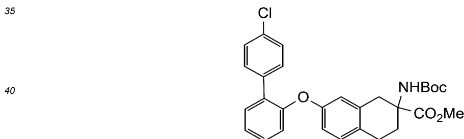
45 methyl 2-((tert-butoxycarbonyl)amino)-7-((4'-chloro-[1,1'-biphenyl]-2-yl)oxy)-1,2,3,4-tetrahydronaphthalene-2-carboxylate
