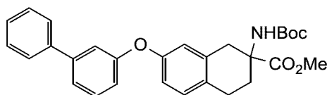
methyl 7-([1,1'-biphenyl]-3-yloxy)-2-((tert-butoxycarbonyl)amino)-1,2,3,4-tetrahydronaphthalene-2-carboxylate
