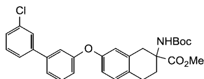
methyl 2-((tert-butoxycarbonyl)amino)-7-((3'-chloro-[1,1'-biphenyl]-3-yl)oxy)-1,2,3,4-tetrahydronaphthalene-2-carboxylate
