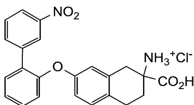
2-carboxy-7-((3'-nitro-[1,1'-biphenyl]-2-yl)oxy)-1,2,3,4-tetrahydronaphthalen-2-aminium chloride
