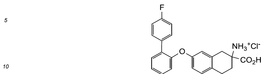
2-carboxy-7-((4'-fluoro-[1,1'-biphenyl]-2-yl)oxy)-1,2,3,4-tetrahydronaphthalen-2-aminium chloride
