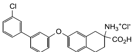
2-carboxy-7-((3'-chloro-[1,1'-biphenyl]-3-yl)oxy)-1,2,3,4-tetrahydronaphthalen-2-aminium chloride
