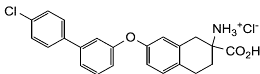
2-carboxy-7-((4'-chloro-[1,1'-biphenyl]-3-yl)oxy)-1,2,3,4-tetrahydronaphthalen-2-aminium chloride
