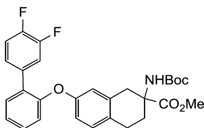
methyl 2-((tert-butoxycarbonyl)amino)-7-((3',4'-difluoro-[1,1'-biphenyl]-2-yl)oxy)-1,2,3,4-tetrahydronaphthalene-2-carboxylate
