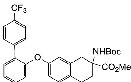
methyl 2-((tert-butoxycarbonyl)amino)-7-((4'-(trifluoromethyl)-[1,1'-biphenyl]-2-yl)oxy)-1,2,3,4-tetrahydronaphthalene-2-carboxylate
