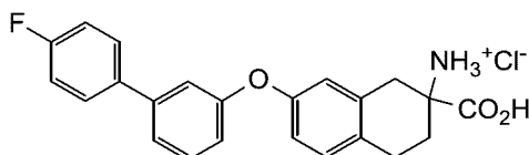
2-carboxy-7-((4'-fluoro-[1,1'-biphenyl]-3-yl)oxy)-1,2,3,4-tetrahydronaphthalen-2-aminium chloride
