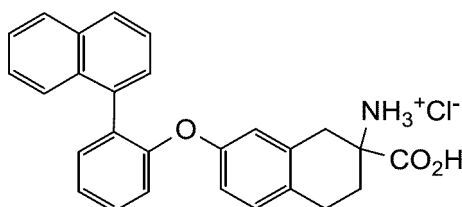
2-carboxy-7-(2-(naphthalen-1-yl)phenoxy)-1,2,3,4-tetrahydronaphthalen-2-aminium chloride
