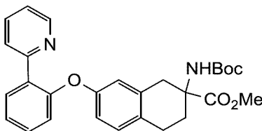
methyl 2-((tert-butoxycarbonyl)amino)-7-(2-(pyridin-2-yl)phenoxy)-1,2,3,4-tetrahydronaphthalene-2-carboxylate
