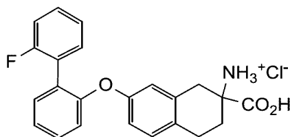
2-carboxy-7-((2'-fluoro-[1,1'-biphenyl]-2-yl)oxy)-1,2,3,4-tetrahydronaphthalen-2-aminium chloride
