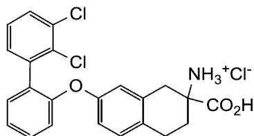
2-carboxy-7-((2',3'-dichloro-[1,1'-biphenyl]-2-yl)oxy)-1,2,3,4-tetrahydronaphthalen-2-aminium chloride
