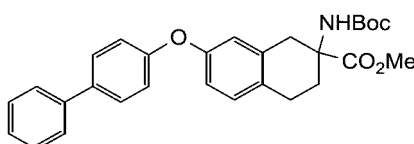
methyl 7-([1,1'-biphenyl]-4-yloxy)-2-((tert-butoxycarbonyl)amino)-1,2,3,4-tetrahydronaphthalene-2-carboxylate
