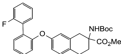
methyl 2-((tert-butoxycarbonyl)amino)-7-((2'-fluoro-[1,1'-biphenyl]-2-yl)oxy)-1,2,3,4-tetrahydronaphthalene-2-carboxylate
