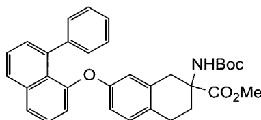
methyl 2-((tert-butoxycarbonyl)amino)-7-((8-phenylnaphthalen-1-yl)oxy)-1,2,3,4-tetrahydronaphthalene-2-carboxylate
