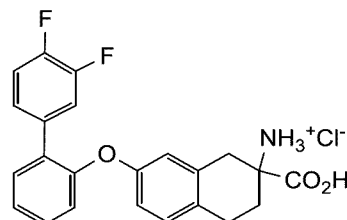
2-carboxy-7-((3',4'-difluoro-[1,1'-biphenyl]-2-yl)oxy)-1,2,3,4-tetrahydronaphthalen-2-aminium chloride
