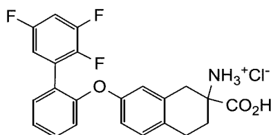
2-carboxy-7-((2',3',5'-trifluoro-[1,1'-biphenyl]-2-yl)oxy)-1,2,3,4-tetrahydronaphthalen-2-aminium chloride
