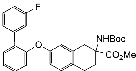
methyl 2-((tert-butoxycarbonyl)amino)-7-((3'-fluoro-[1,1'-biphenyl]-2-yl)oxy)-1,2,3,4-tetrahydronaphthalene-2-carboxylate
