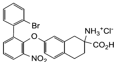
7-((2'-bromo-3-nitro-[1,1'-biphenyl]-2-yl)oxy)-2-carboxy-1,2,3,4-tetrahydronaphthalene-2-aminium chloride
