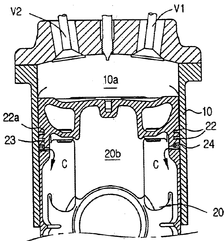
FIG. 1C PRIOR ART
