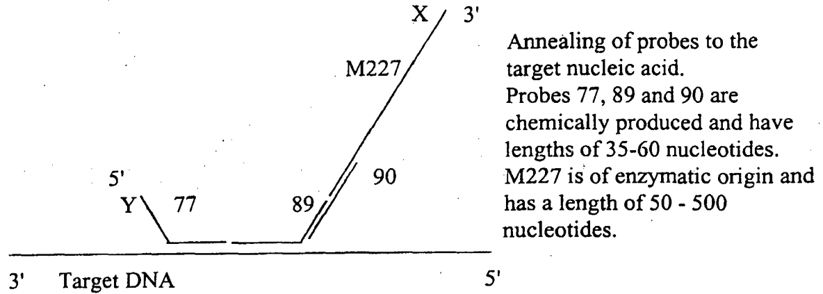
FIGURE 12 : The use of the MLPA invention without the use of target specific clones.
