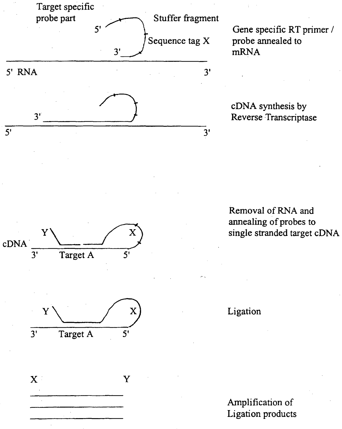
FIGURE 11 : The use of reverse transcriptase primers that are part of one of the probes.
