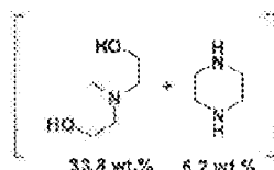
DMDEA
