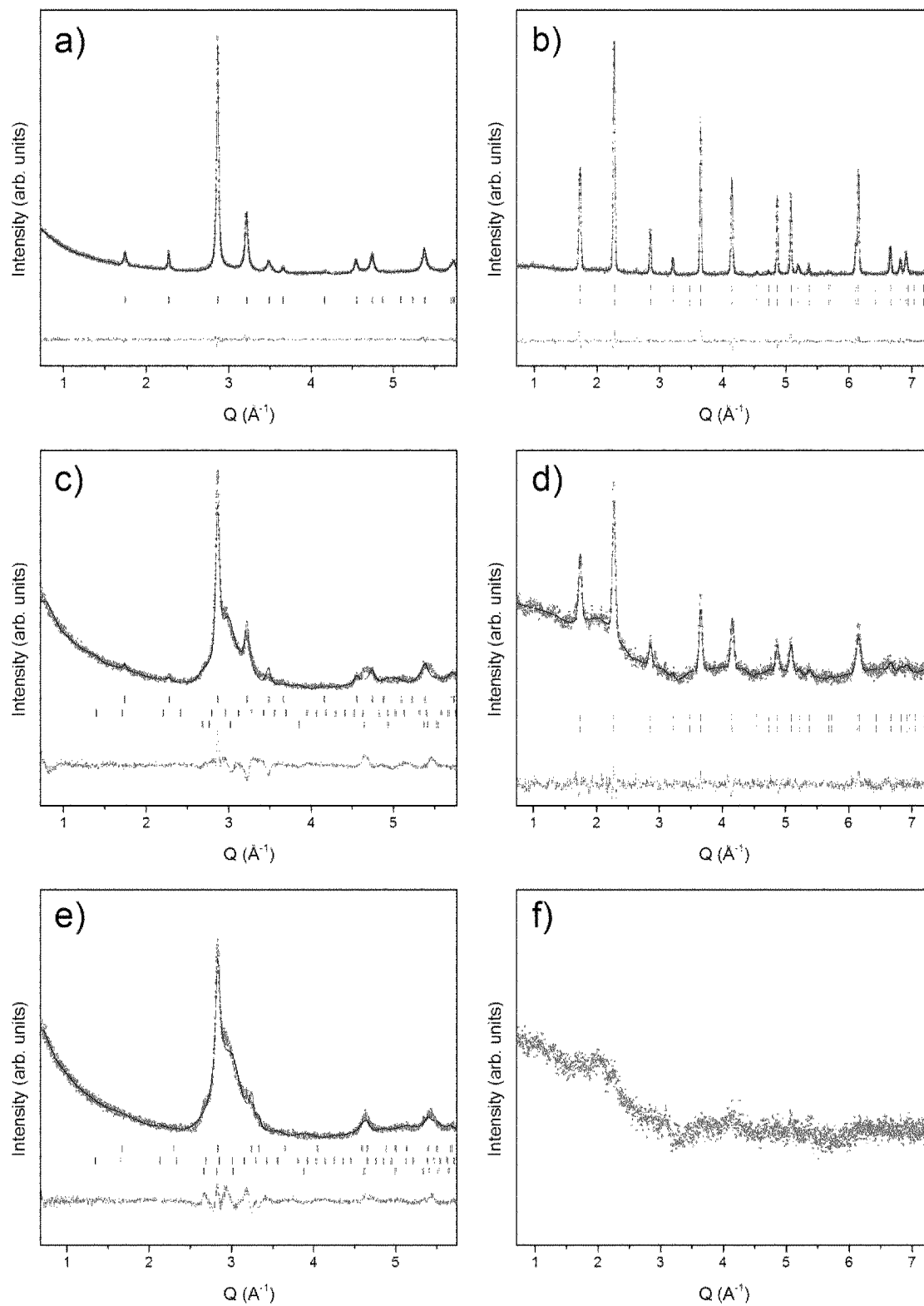
Figure 3: XRD and NPD patterns before flash heating
