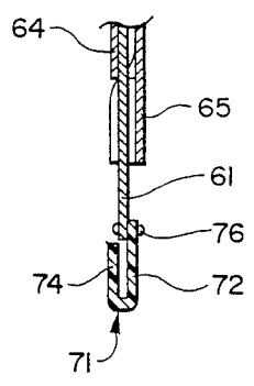
FIG. 3 PRIOR ART
