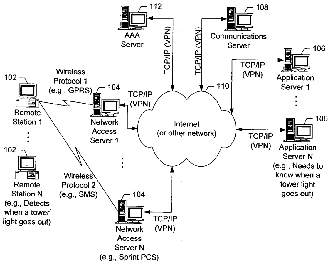
Communications System 100
