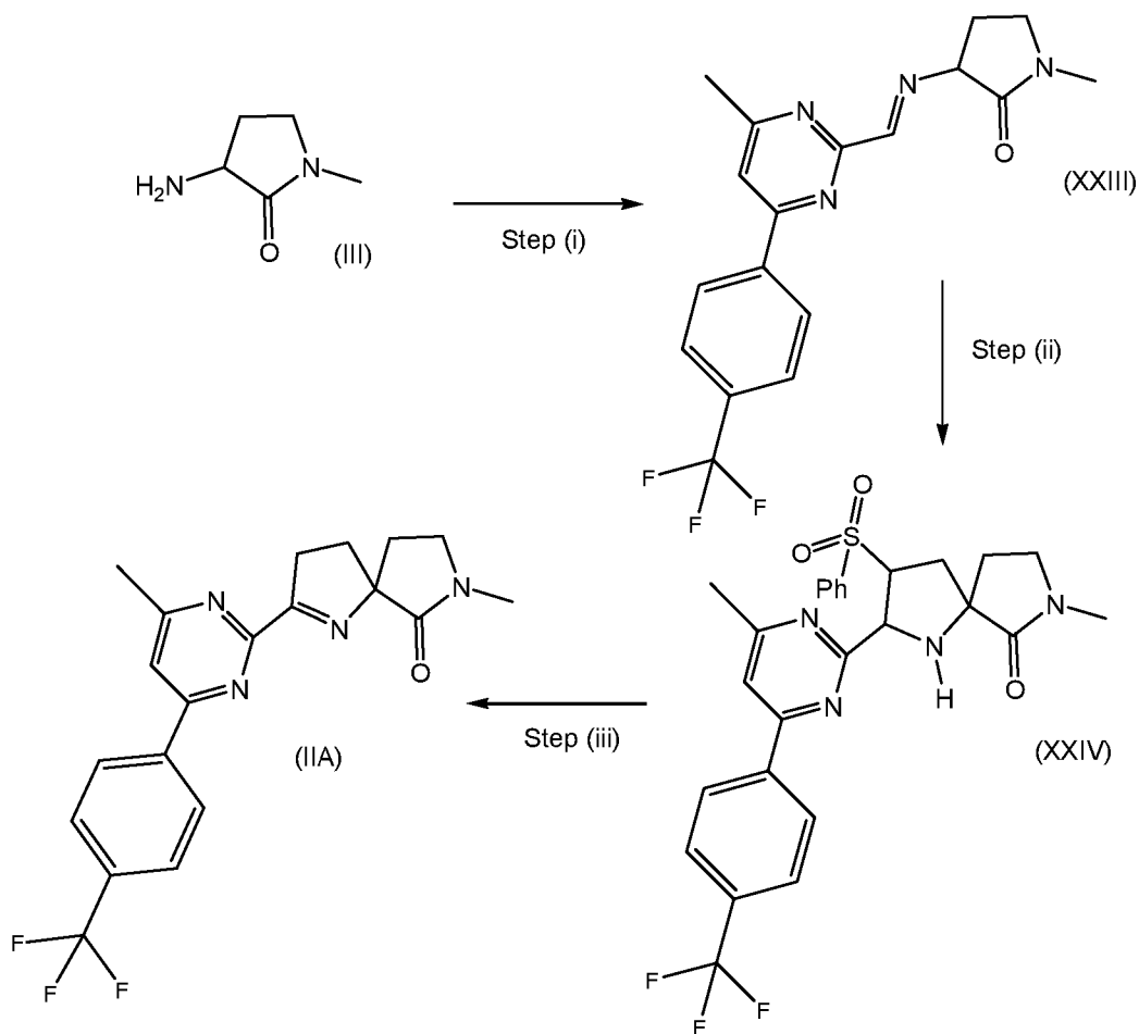
Scheme 3
