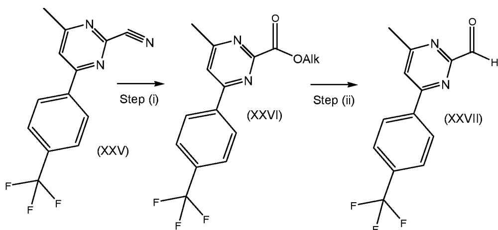
Scheme 4
