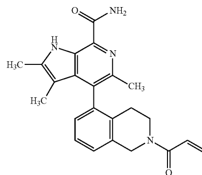
Atropisomers 1 and 2
