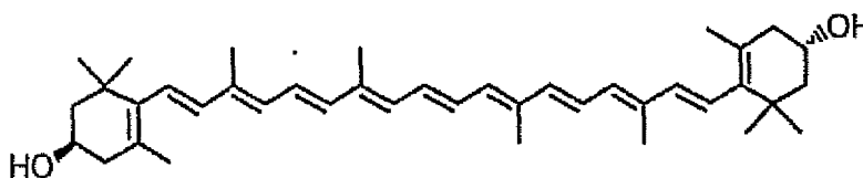
Fig 2: Zeaxanthin, ((3R,3'R)- \beta,\beta carotene-3,3'-diol)
