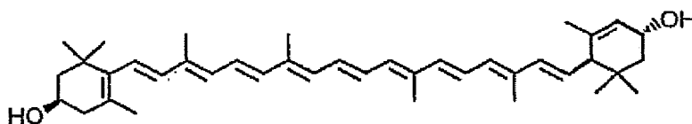
Fig. 1: Lutein, (3R,3'R,6'R)- \beta,\epsilon -carotene-3,3'-diol)
