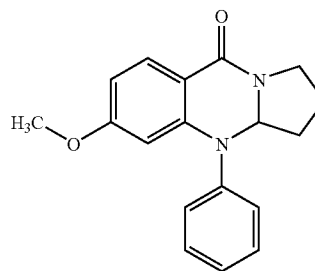
6-methoxy-4-phenyl-2,3,3a,4-tetrahydropyrrolo[2,1-b]quinazolin-9(1H)-one
