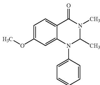
7-methoxy-2,3-dimethyl-1-phenyl-2,3-dihydroquinazolin-4(1H)-one
