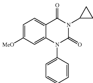
3-cyclopropyl-7-methoxy-1-phenylquinazoline-2,4-dione
