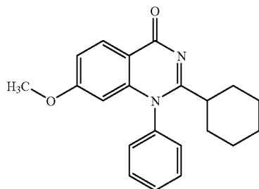
2-cyclohexyl-7-methoxy-1-phenylquinazolin-4(1H)-one
