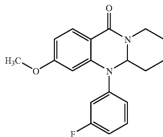
5-(3-fluorophenyl)-3-methoxy-5,5a,6,7,8,9-hexahydro-11H-pyrido[2,1-b]quinazolin-11-one
