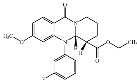
(5,6-cis)-5-(3-fluorophenyl)-3-methoxy-11-oxo-5,6,7,8,9,11-hexahydro-5aH-pyrido[2,1-b]quinazoline-6-carboxylate
