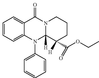
ethyl (5,6-cis)-11-oxo-5-phenyl-5,6,7,8,9,11-hexahydro-5aH-pyrido[2,1-b]quinazoline-6-carboxylate
