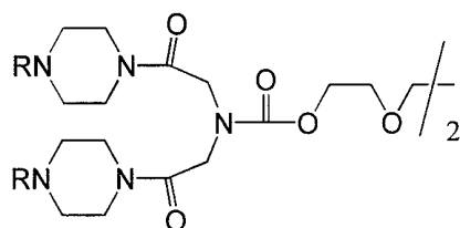
Platform (bromoacetyl-PITG)
