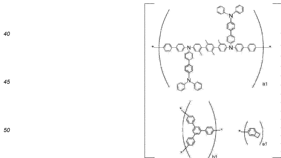
[Copolymer Type 20]
