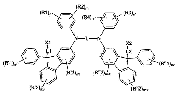
[Chemical Formula 1]
