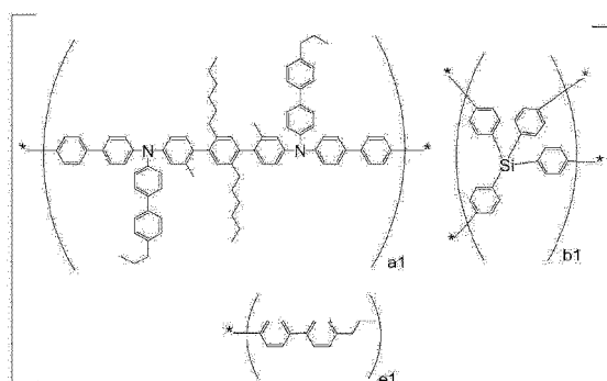
[Copolymer Type 14]
