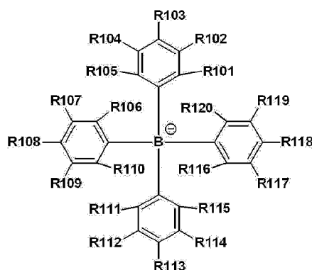
[Chemical Formula 2]
