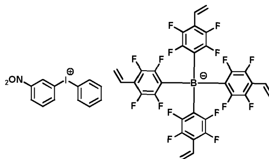
[Chemical Formula 1-1-12]
