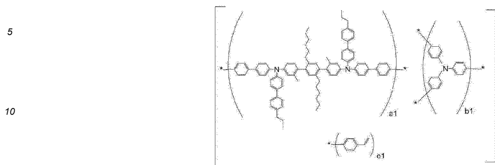
[Copolymer Type 18]
