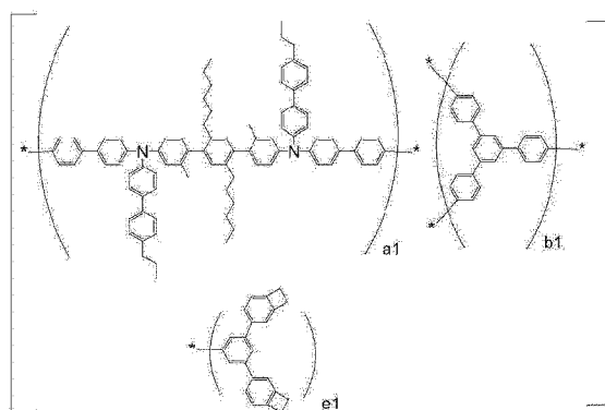
[Copolymer Type 6]
