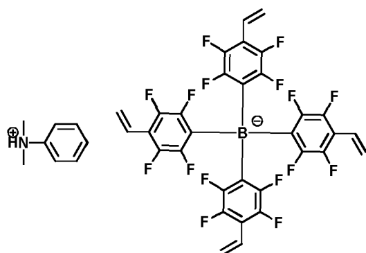
[Chemical Formula 1-1-34]
