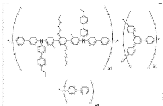
[Copolymer Type 2]
