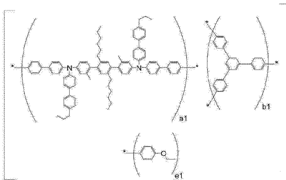
[Copolymer Type 11]
