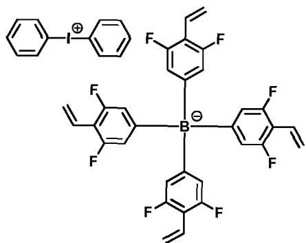
[Chemical Formula 1-1-25]
