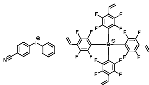
[Chemical Formula 1-1-13]
