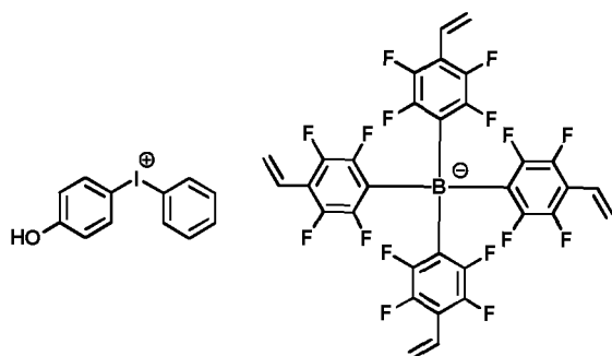
[Chemical Formula 1-1-7]
