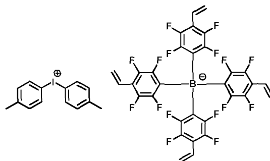
[Chemical Formula 1-1-6]
