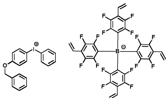
[Chemical Formula 1-1-7]
