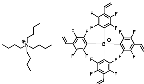
[Chemical Formula 1-1-36]
