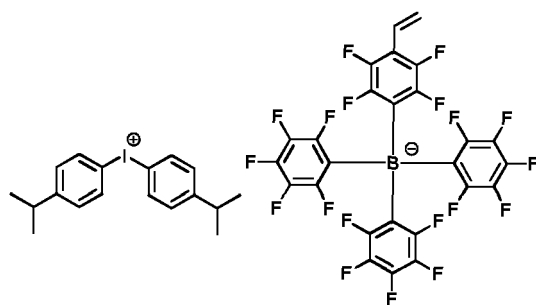
[Chemical Formula 1-1-15]
