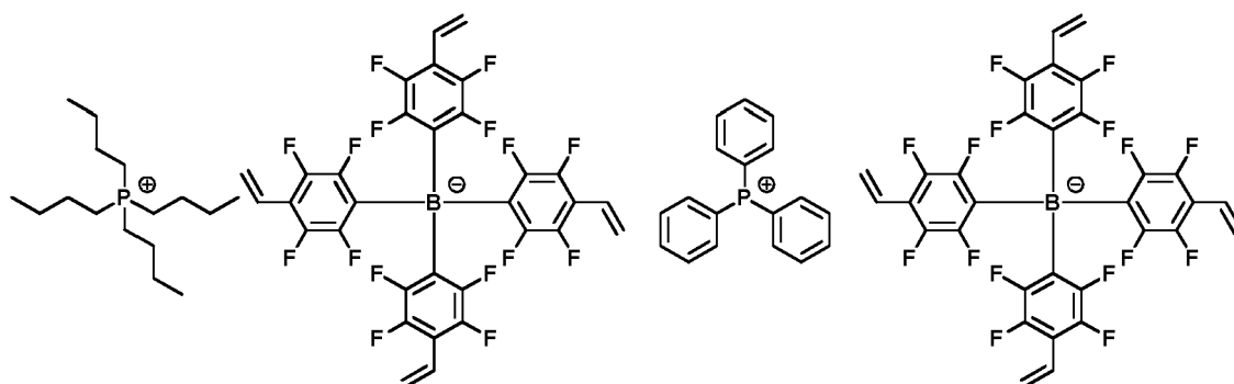
[Chemical Formula 1-1-29]
