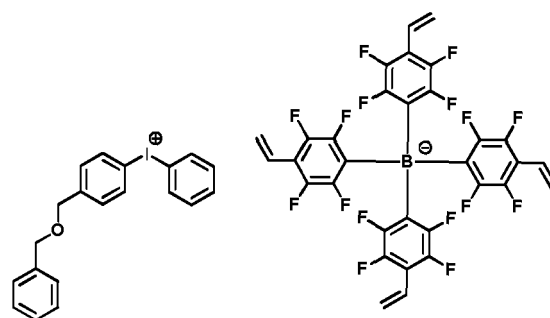
[Chemical Formula 1-1-14]
