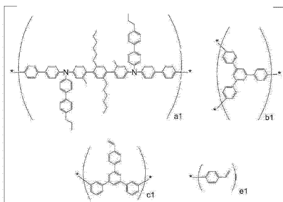
[Copolymer Type 10]
