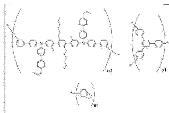
[Copolymer Type 15]
