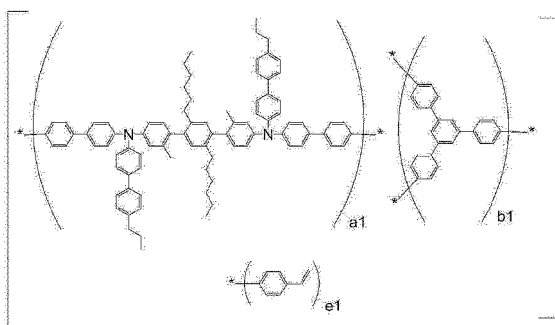
[Copolymer Type 8]
