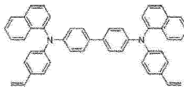
[Comparative Compound 2]
