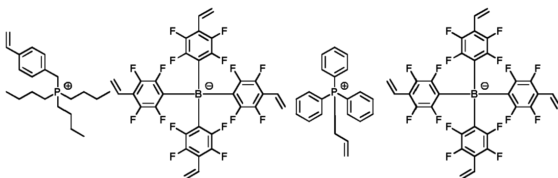
[Chemical Formula 1-1-29]
