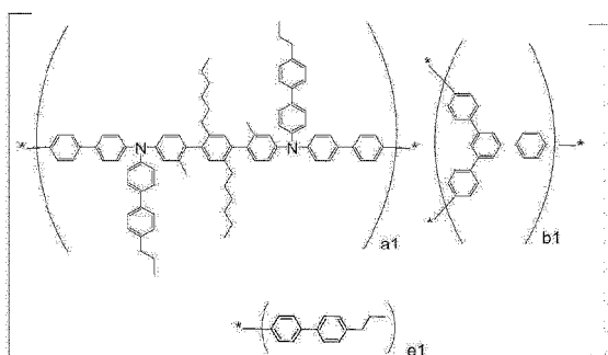
[Copolymer Type 7]
