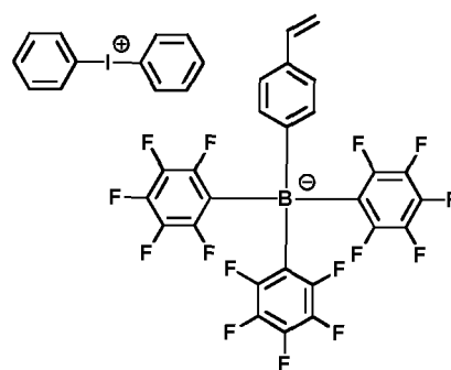
[Chemical Formula 1-1-20]
