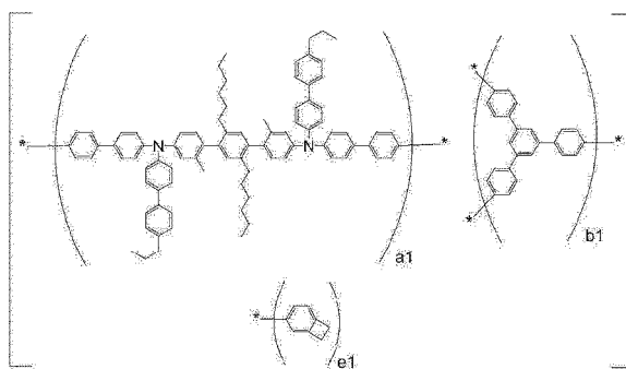
[Copolymer Type 1]
