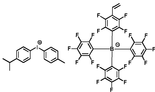
[Chemical Formula 1-1-15]
