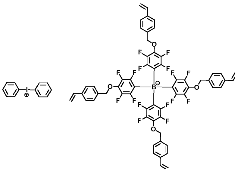
[Chemical Formula 1-1-26]
