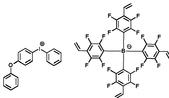
[Chemical Formula 1-1-8]
