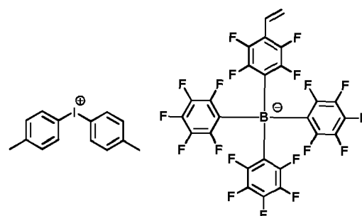
[Chemical Formula 1-1-16]
