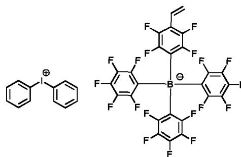
[Chemical Formula 1-1-16]
