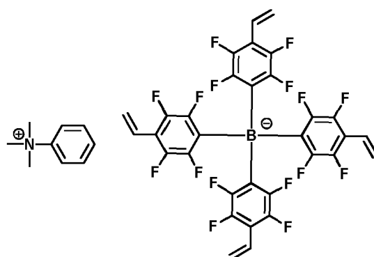
[Chemical Formula 1-1-33]
