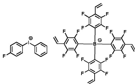
[Chemical Formula 1-1-11]
