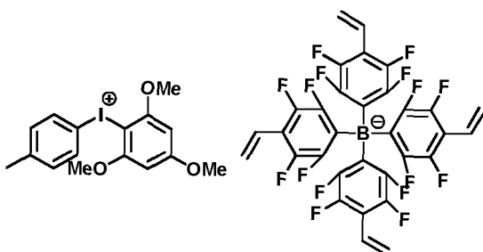
[Chemical Formula 1-1-21]
