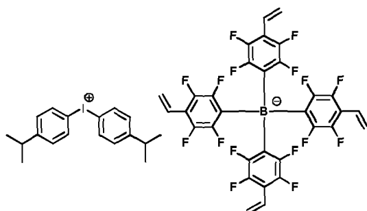
[Chemical Formula 1-1-5]
