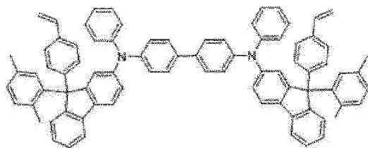
[Comparative Compound 1]
