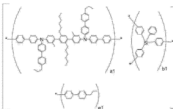
[Copolymer Type 13]
