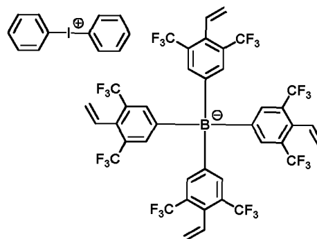
[Chemical Formula 1-1-24]
