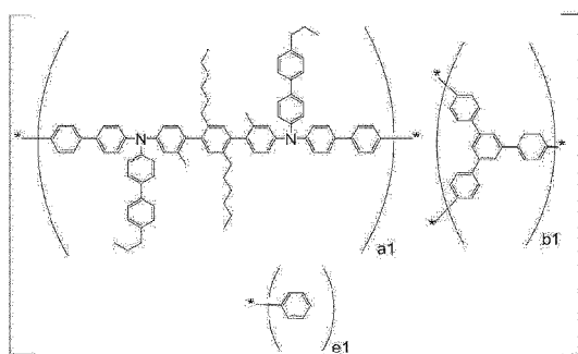
[Copolymer Type 9]
