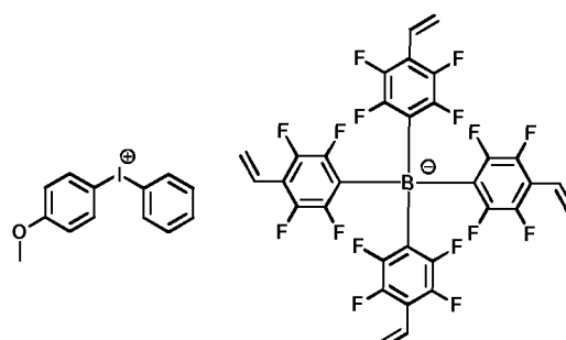
[Chemical Formula 1-1-8]
