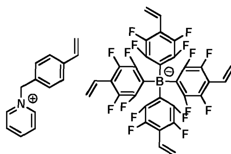
[Chemical Formula 1-1-37]
