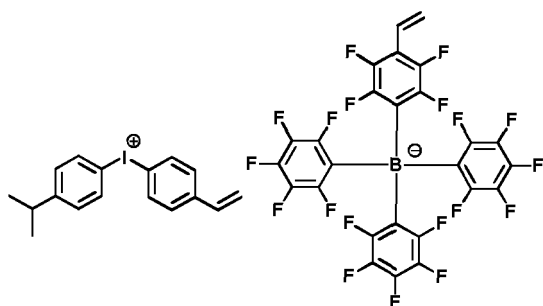
[Chemical Formula 1-1-19]
