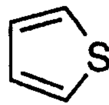
thiophene (thienyl)
