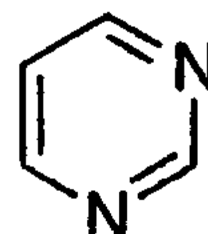
pyrimidine (pyrimidinyl)
