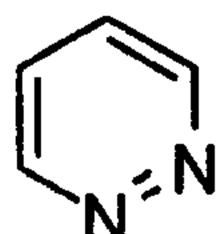
pyridazine (pyridazinyl)
