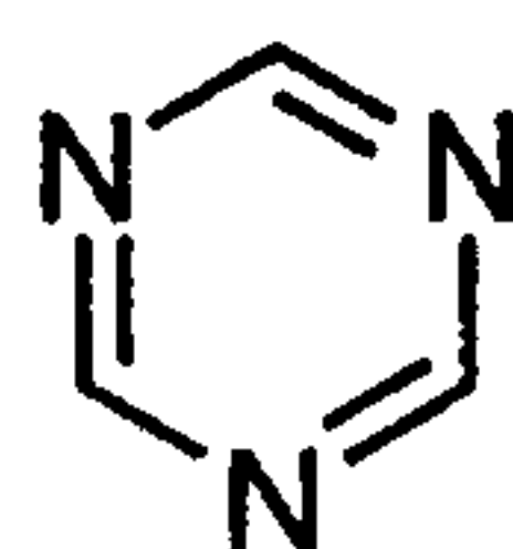
triazine (triazinyl)
