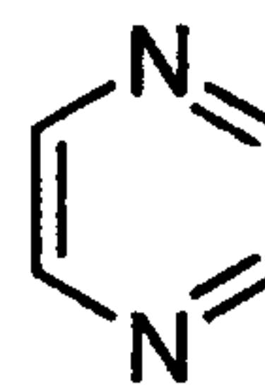
pyrazine (pyrazinyl)
