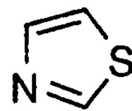
thiazole (thiazolyl)
