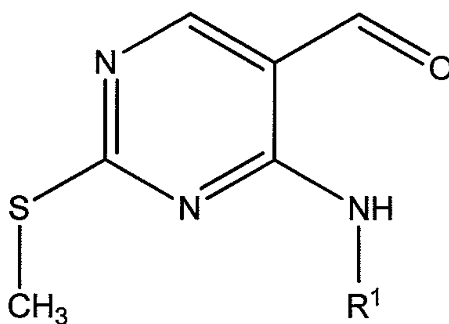
Formula IV
