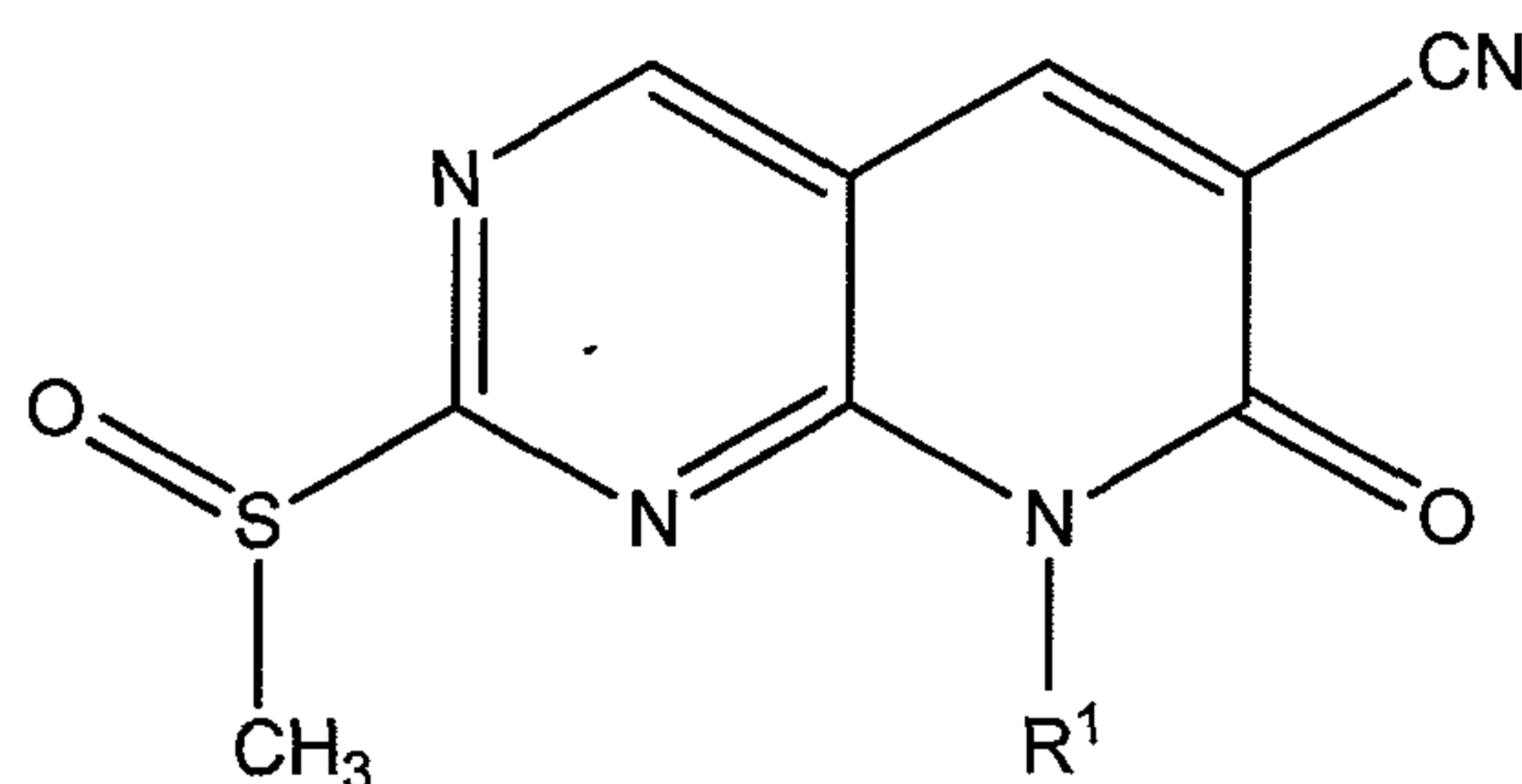
Formula II
