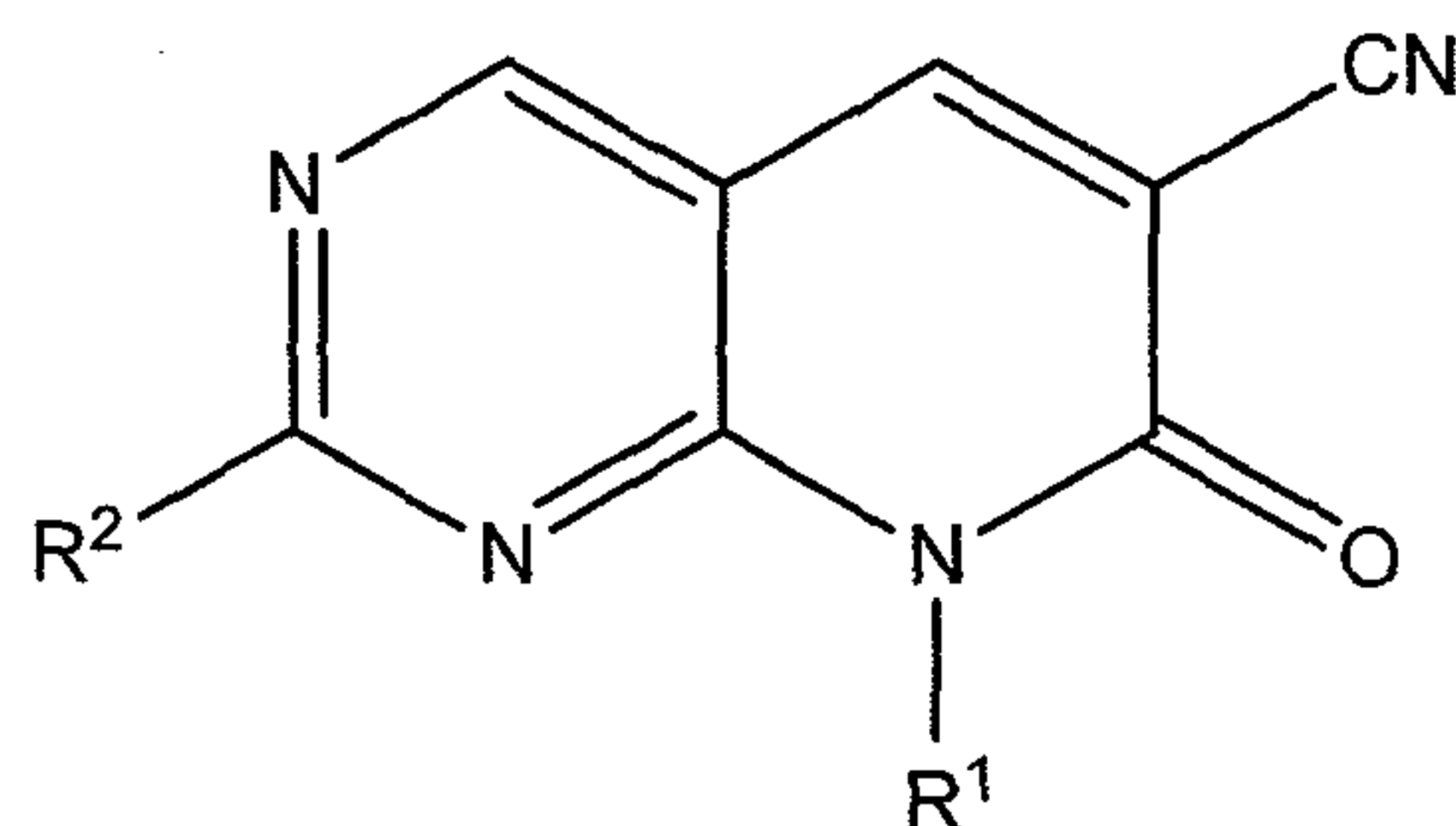
Formula I
