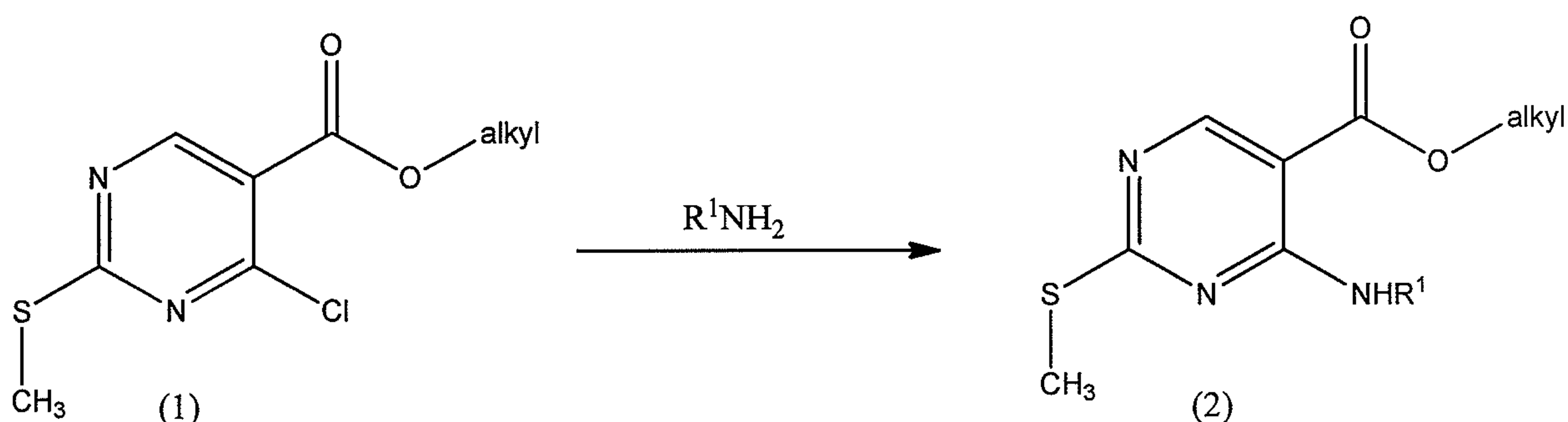
Scheme 1
