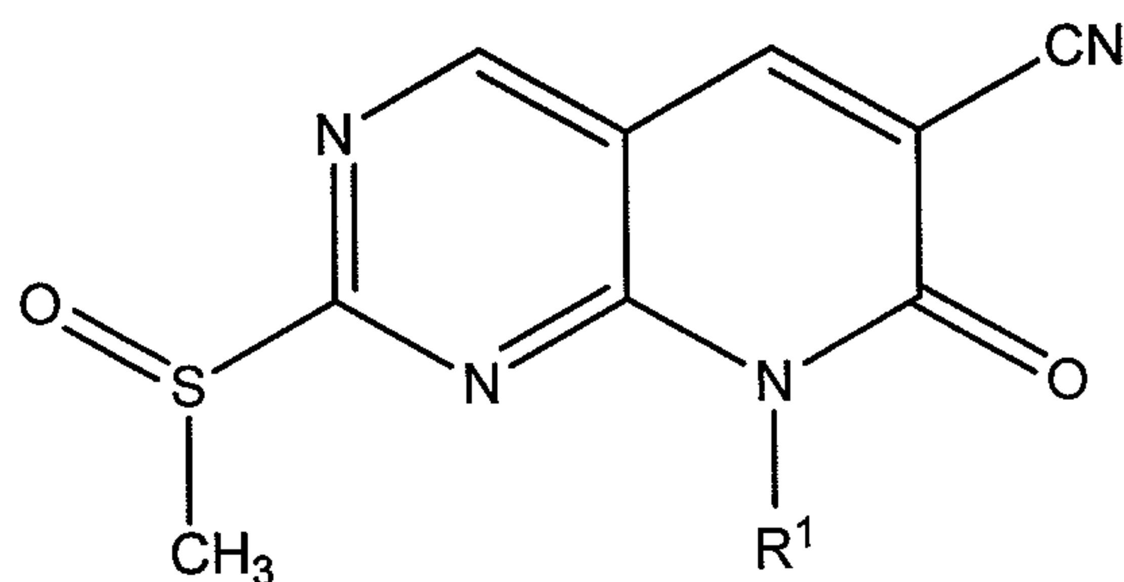
Formula II
