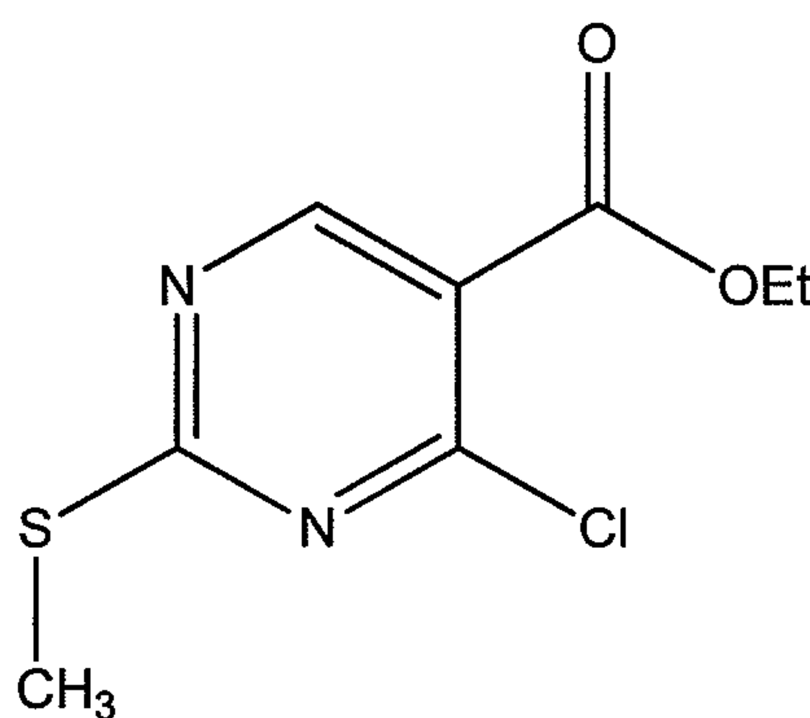
Formula VII
