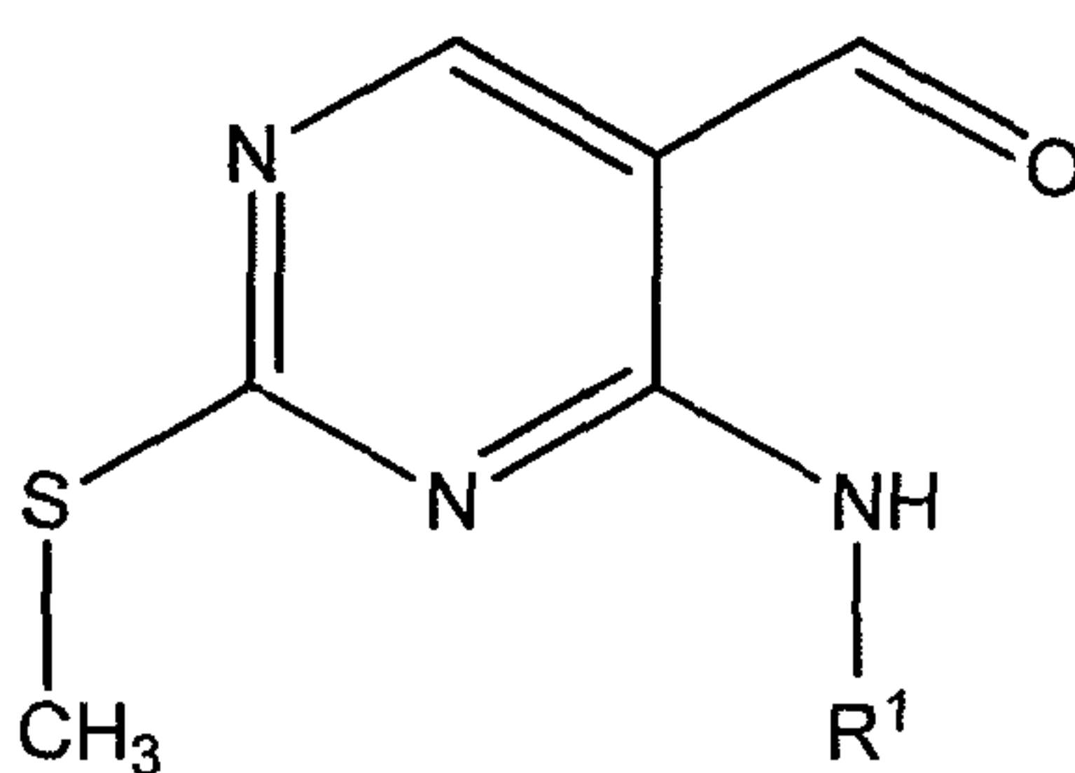
Formula IV
