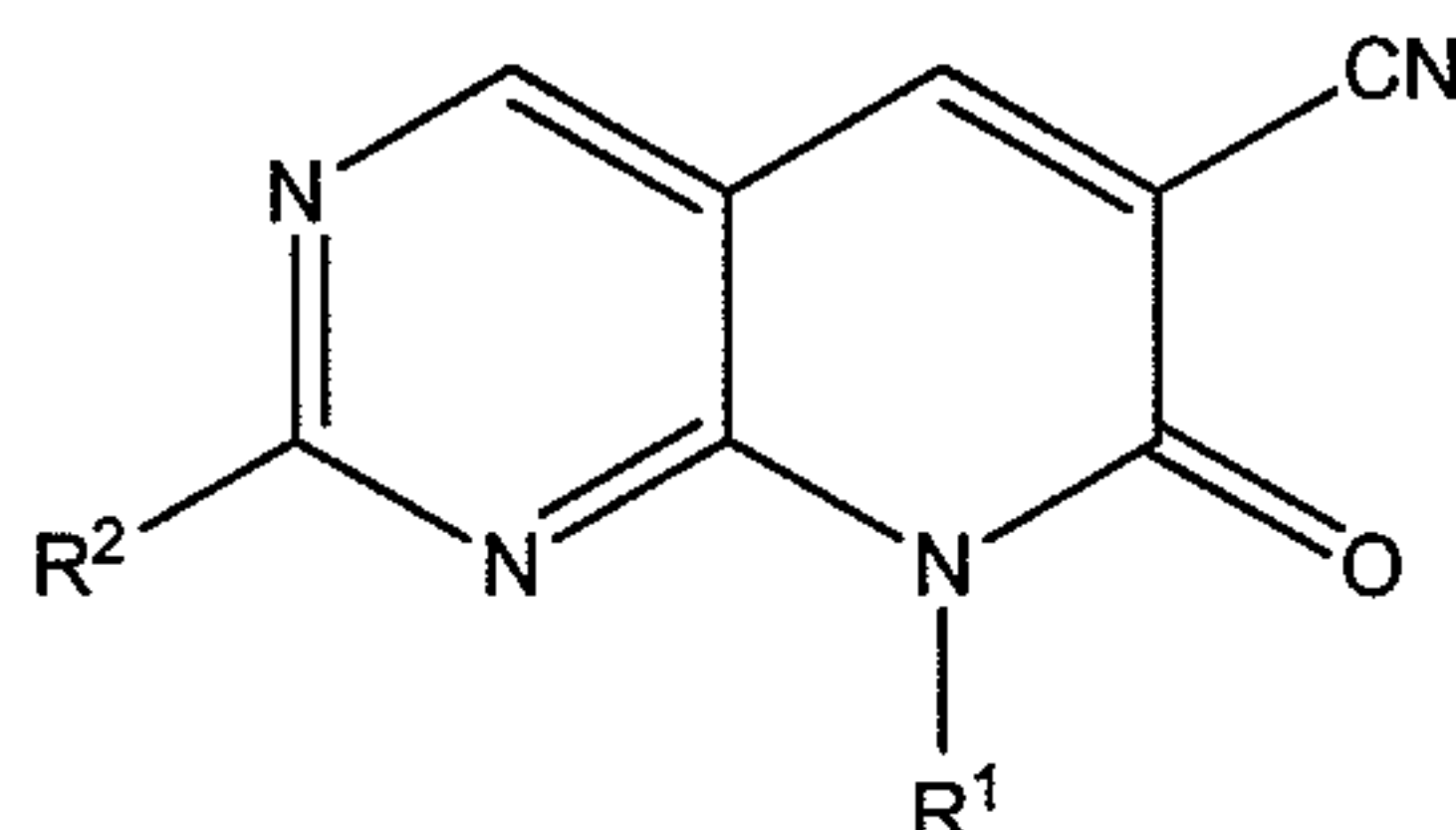
Formula I.
