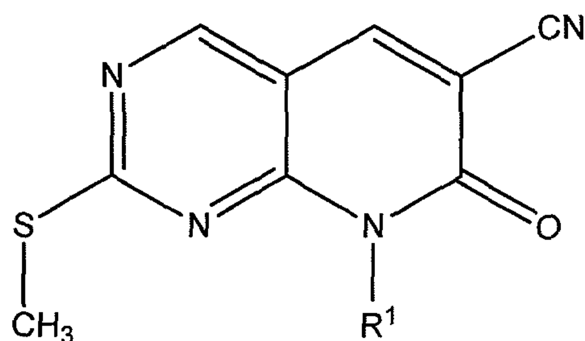
Formula III
