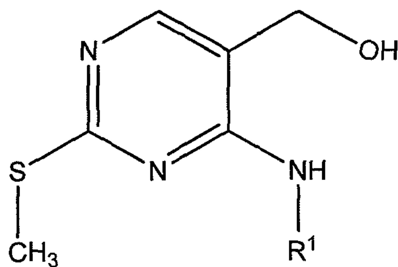
Formula V.
