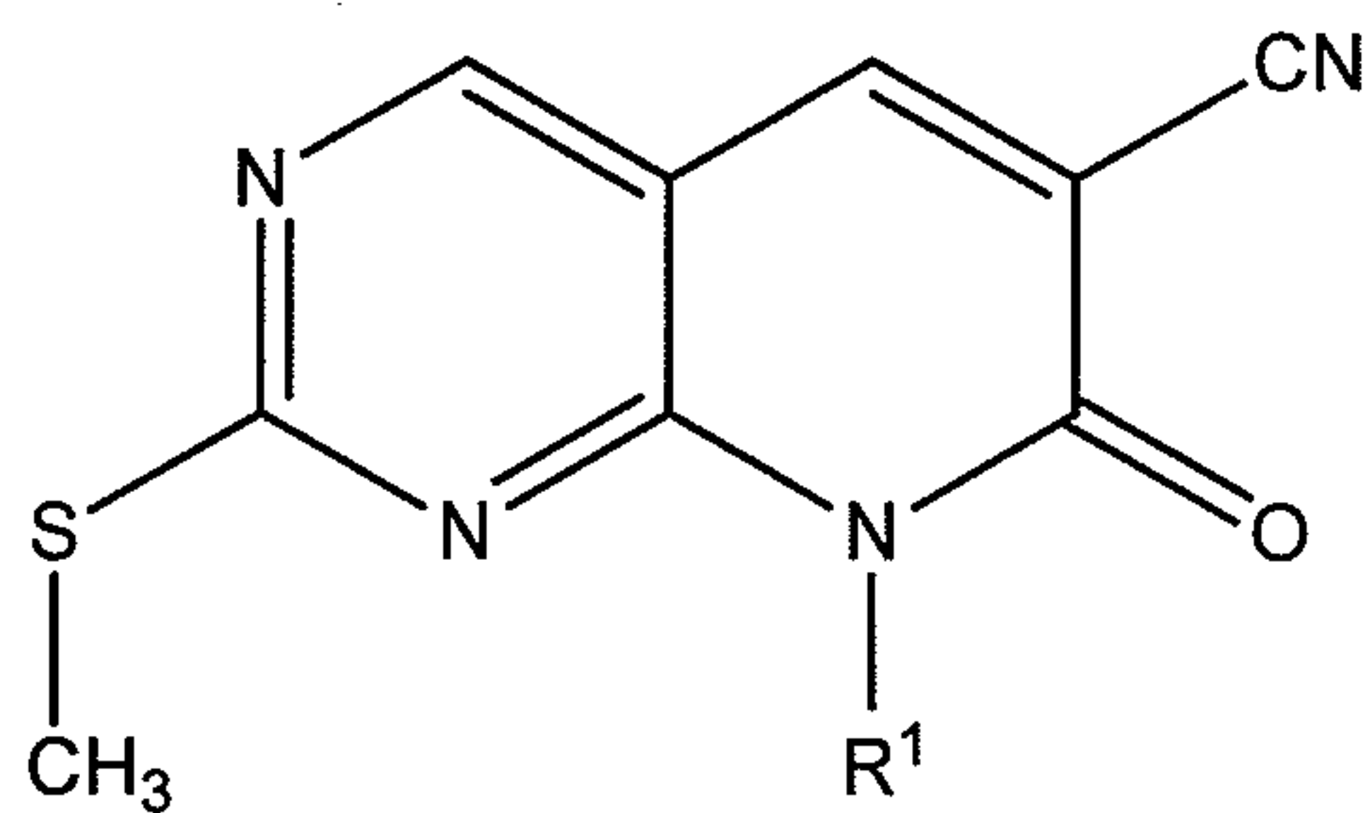
Formula III
