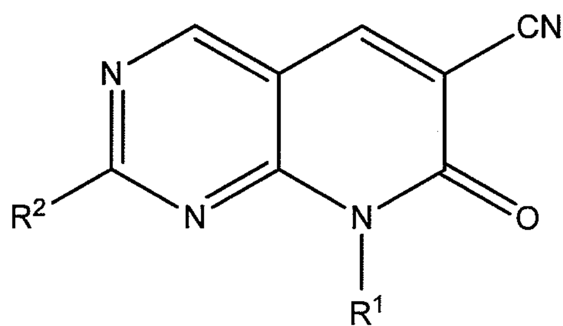
Formula I
