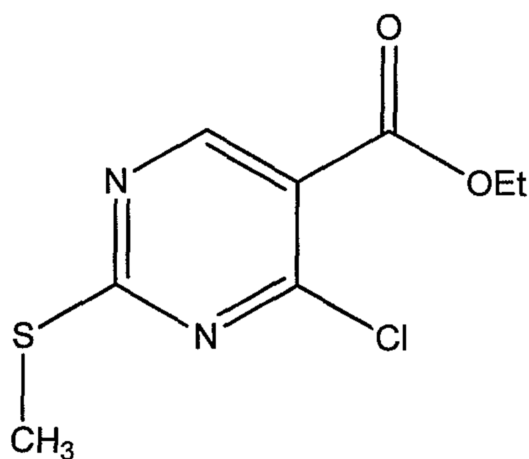
Formula VII
