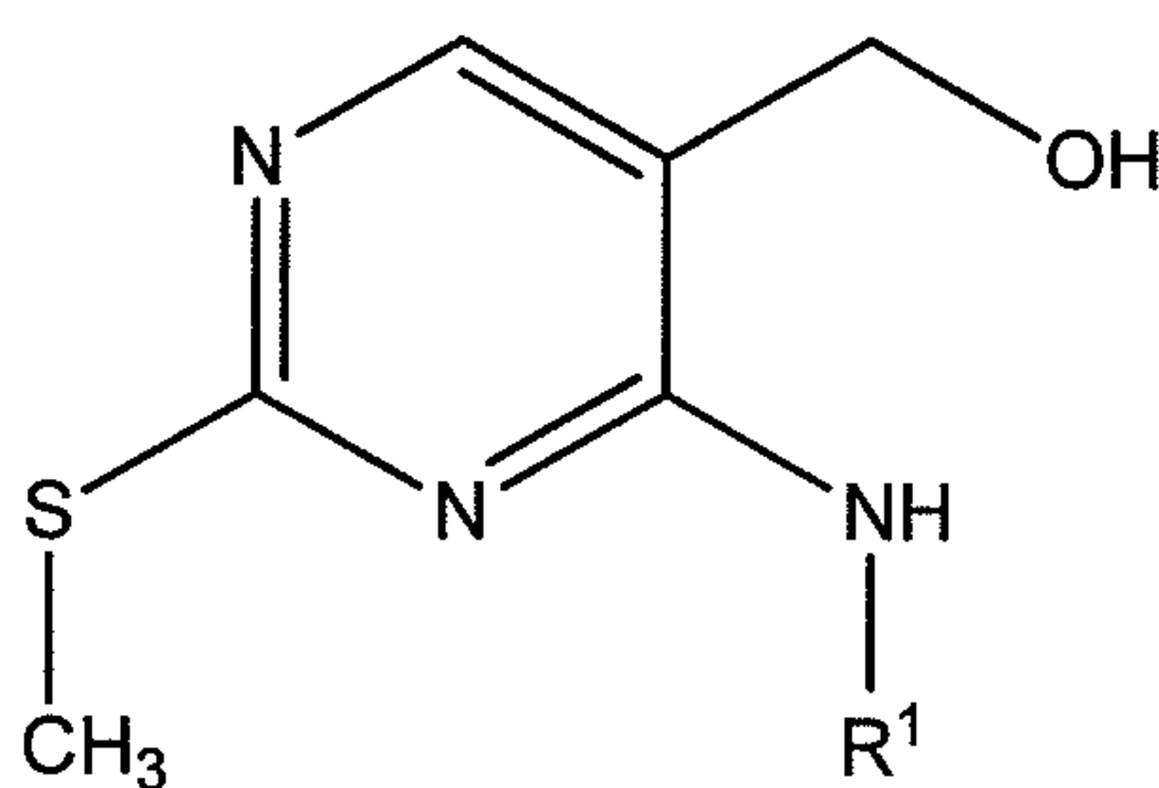
Formula V.
