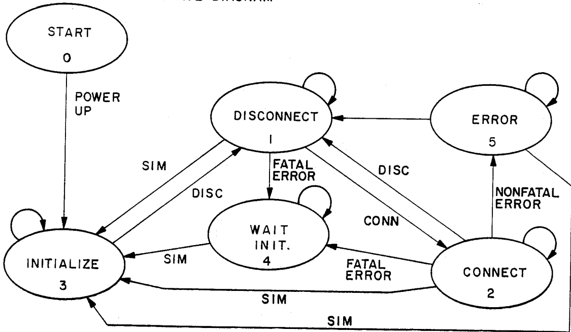
FIG 27 SECONDARY STATION CONNECTION STATE DIAGRAM
