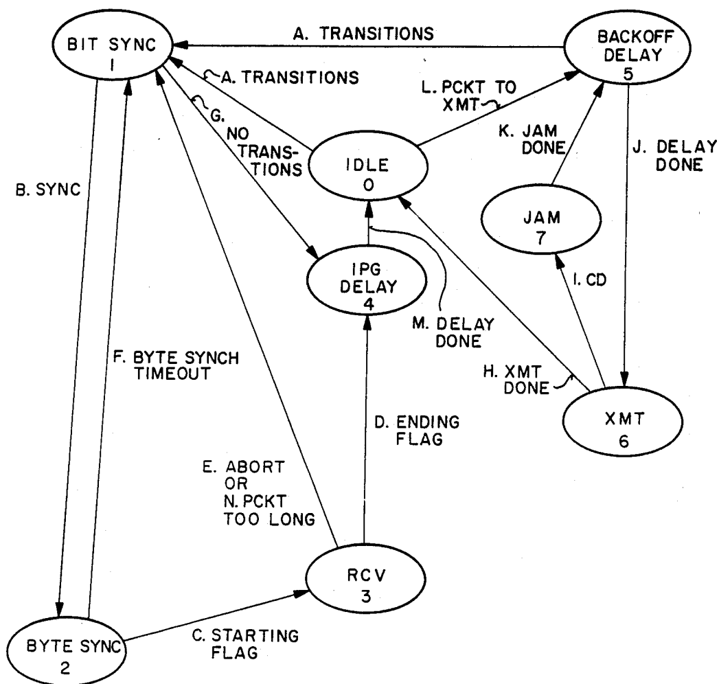
CONTENTION &amp; I/O STATE DIAGRAM
