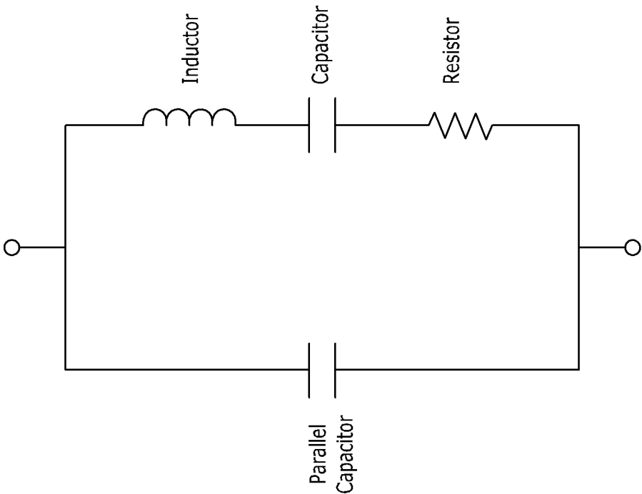
Components of Piezoelectric Transducer in a circuit
