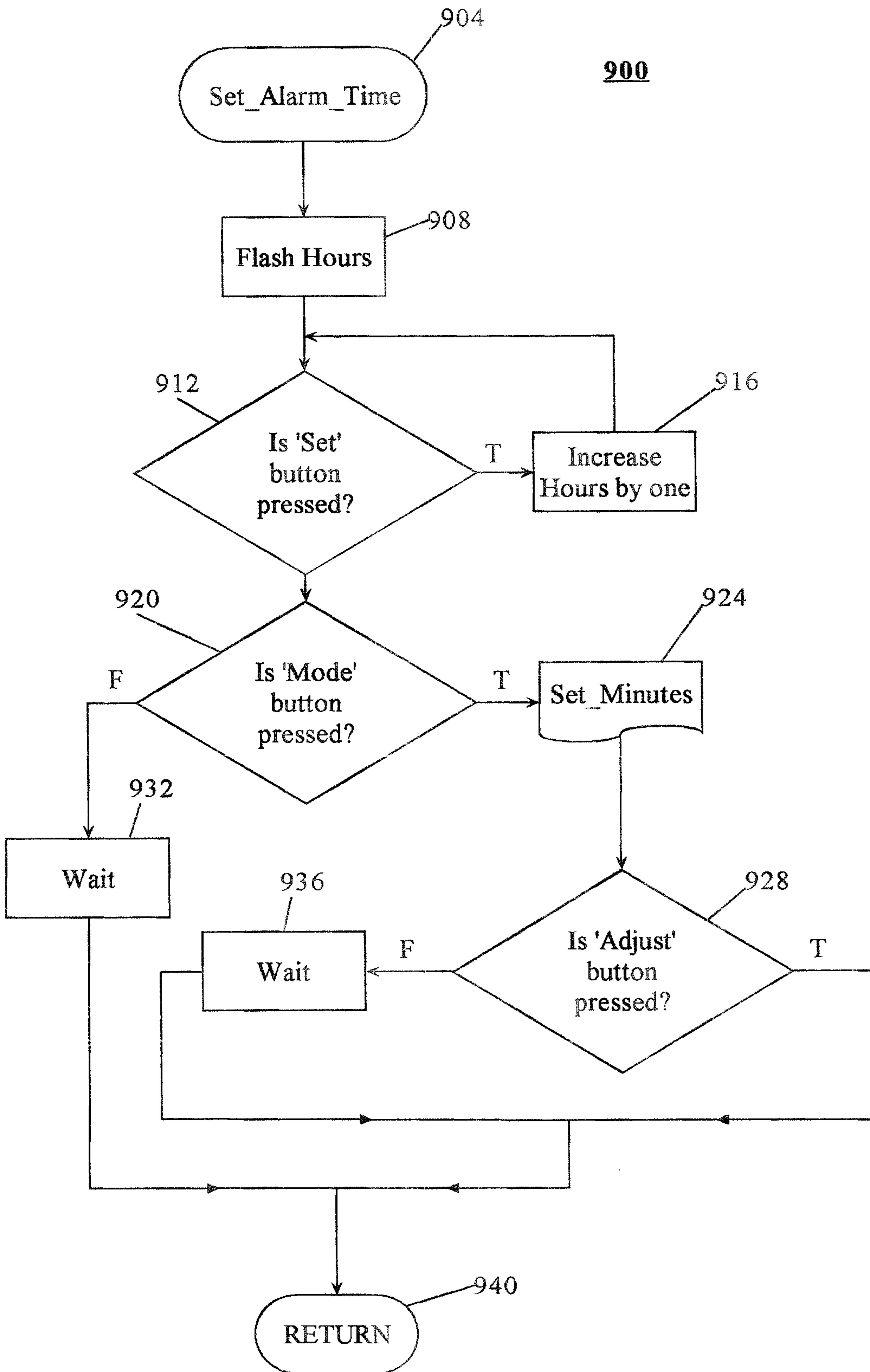
FIG. 9 Setting Alarm Time Sub-Procedure
