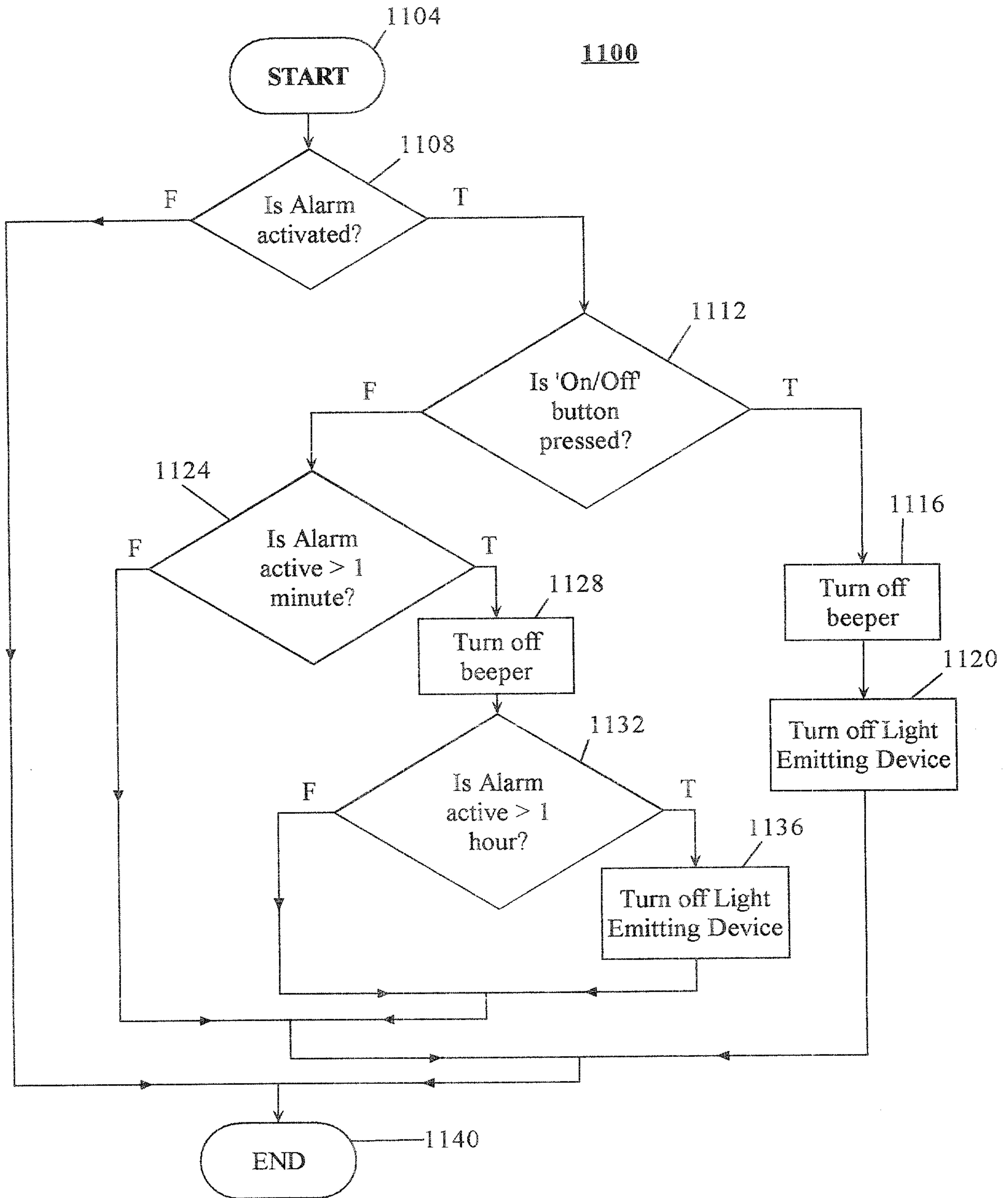
FIG. 11 Resetting Active Alarm
