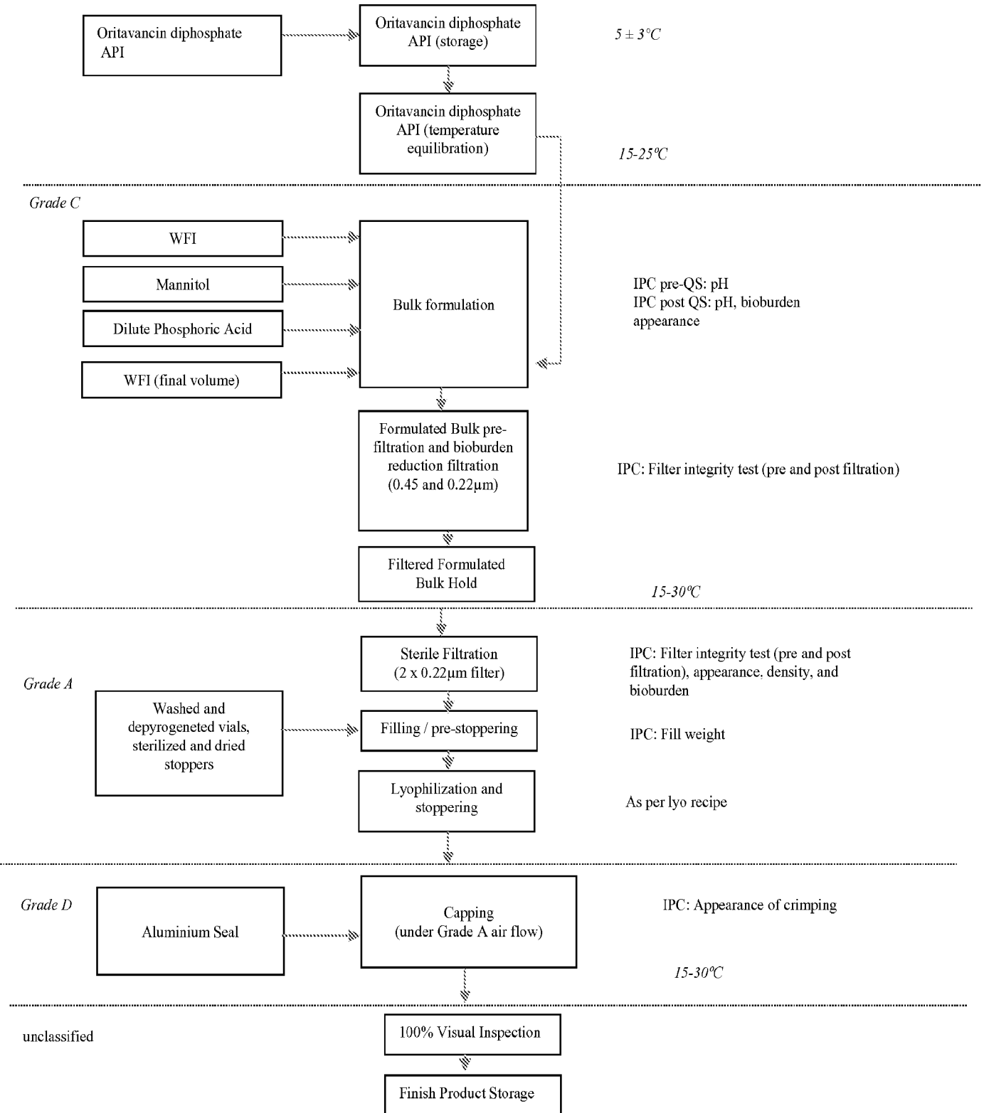
Figure 6 - Schematic Process Flow Diagram of Manufacturing Process
