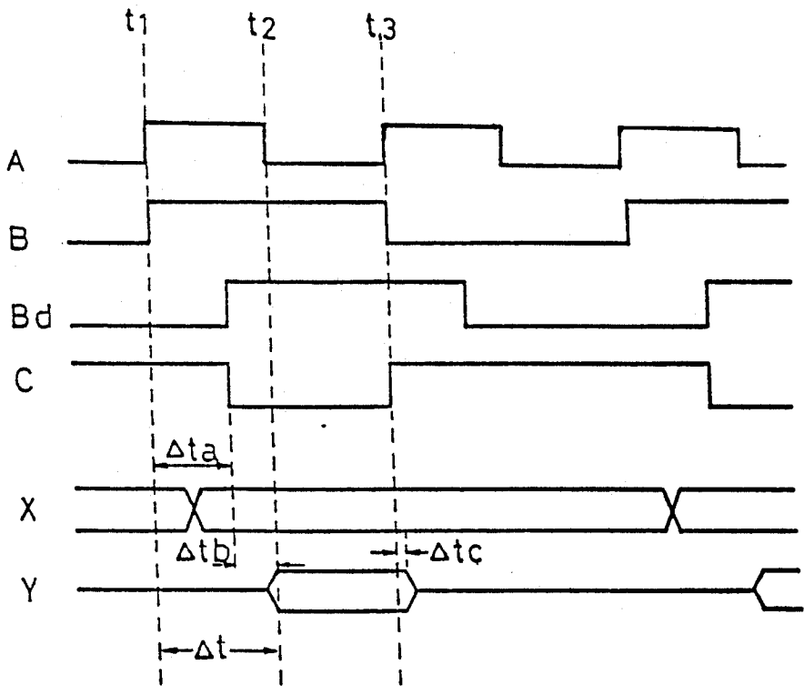
FIG. 5 PRIOR ART
