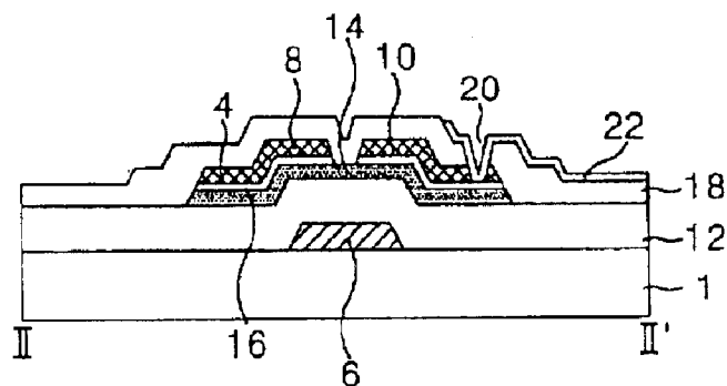
FIG. 2 RELATED ART
