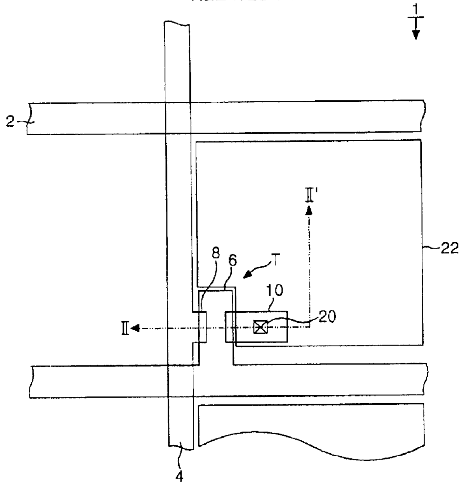
FIG. 1 RELATED ART
