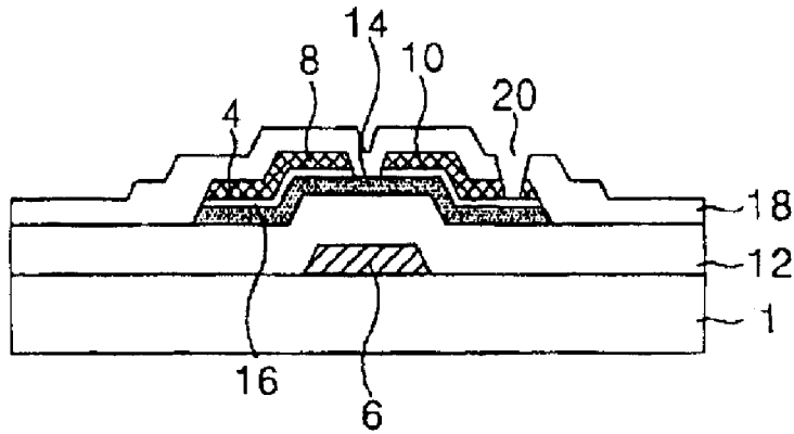
FIG. 3C RELATED ART
