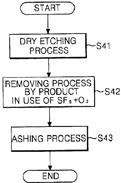
FIG. 4 RELATED ART
