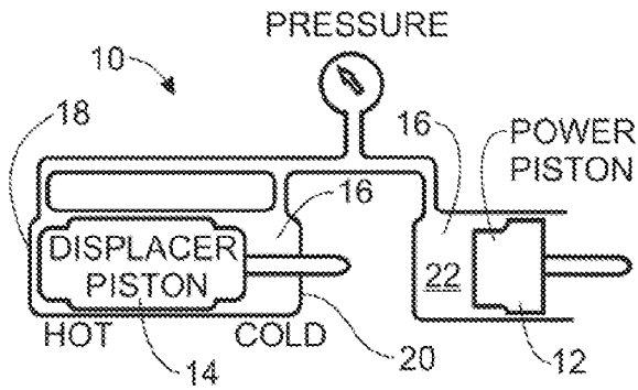
READY FOR START OF COMPRESSION STROKE
