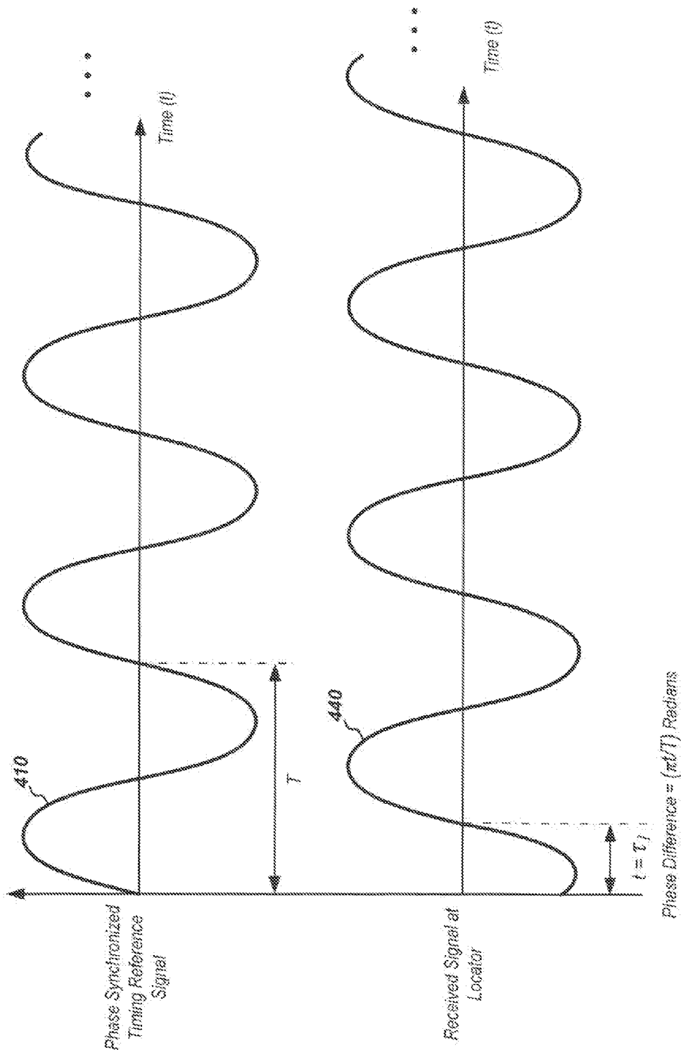
FIG. 4C Example Current Signaling in Buried Object with Phase Shift Caused by Coupling Impedance
