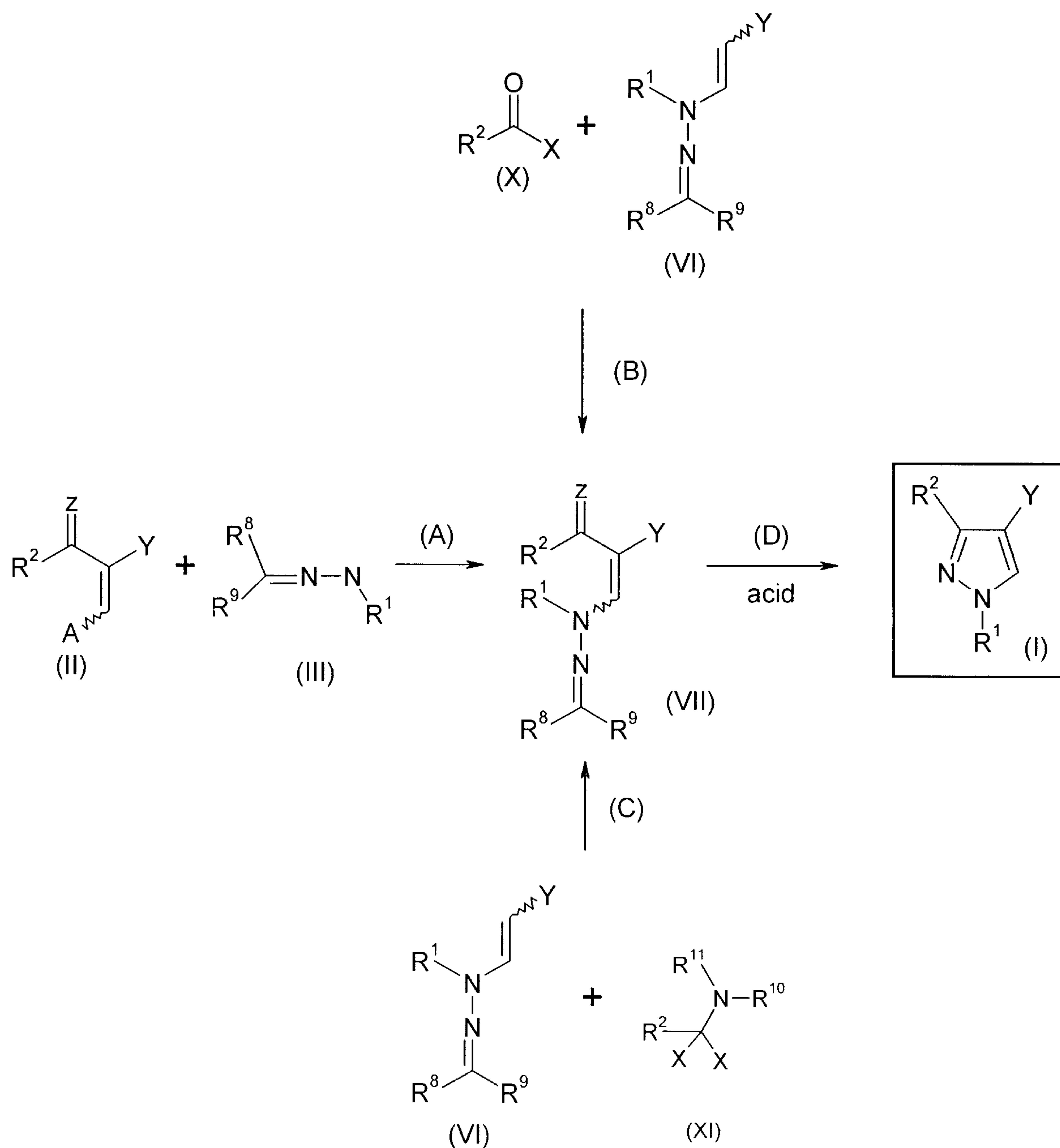
Scheme 3
