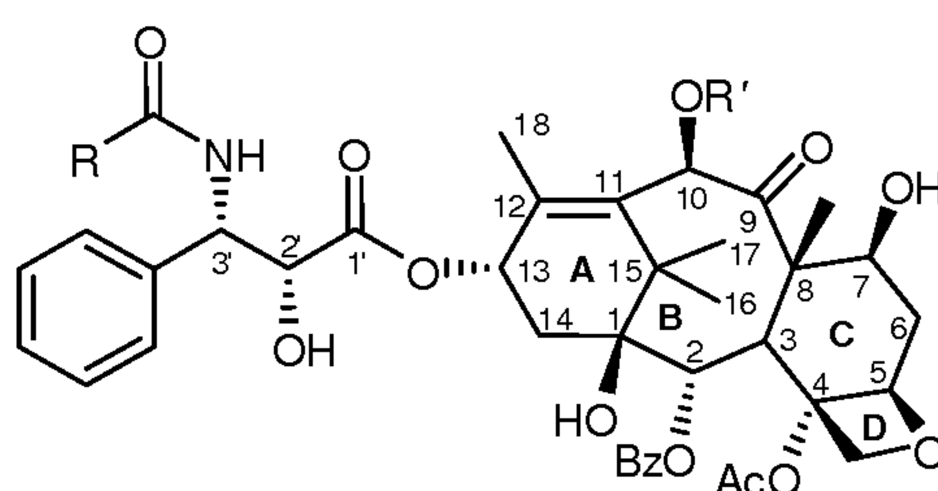
Paclitaxel: R = \text{Ph} ; R' = \text{acetyl} Docetaxel: R = -\text{OtBu} ; R' = \text{H}
