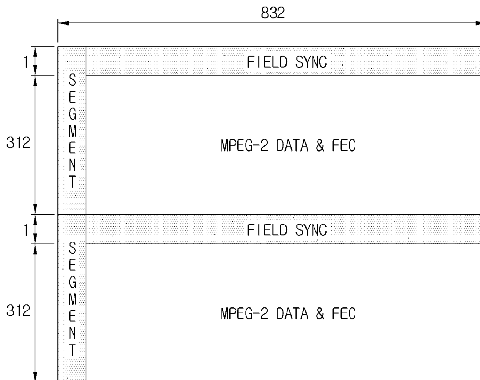
FIG. 2 (PRIOR ART)
